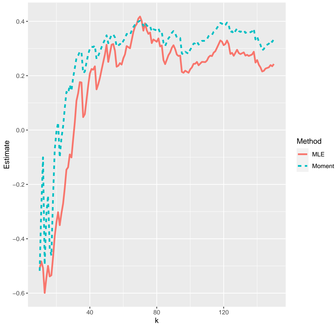
Estimates of extreme value index--18-08-2020
