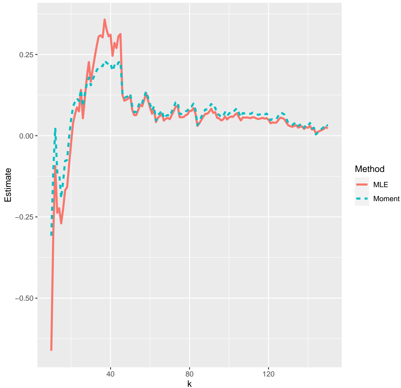
Estimates of extreme value index--18-05-2021
