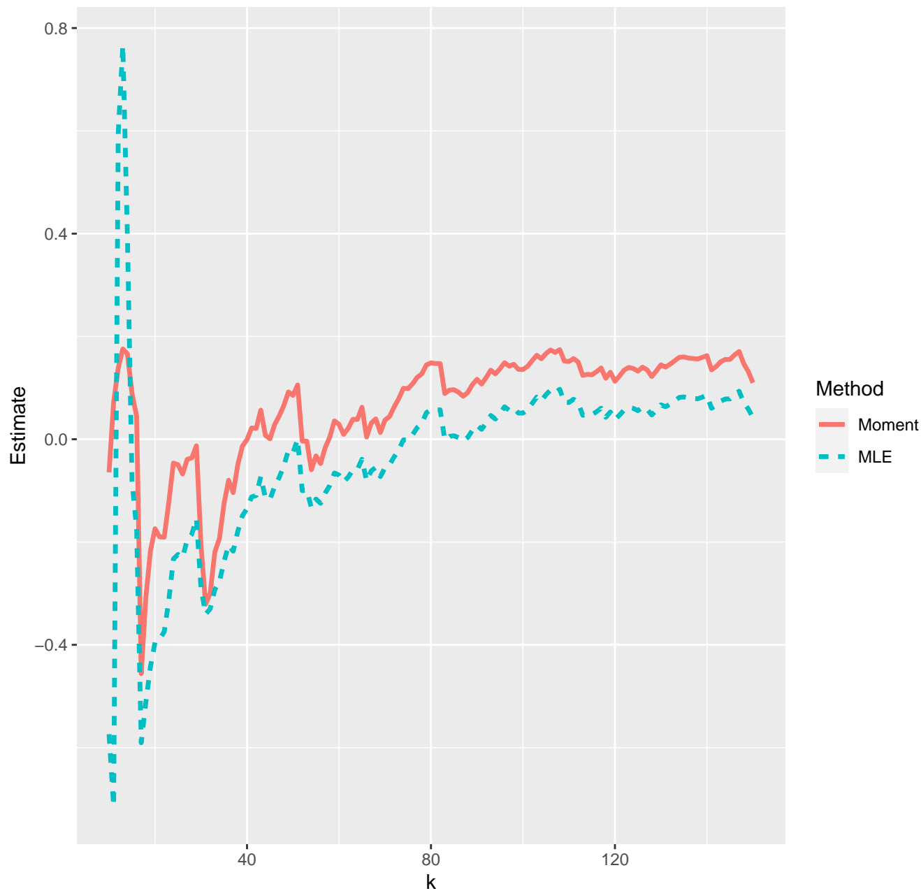
Estimates of extreme value index--18-04-2020
