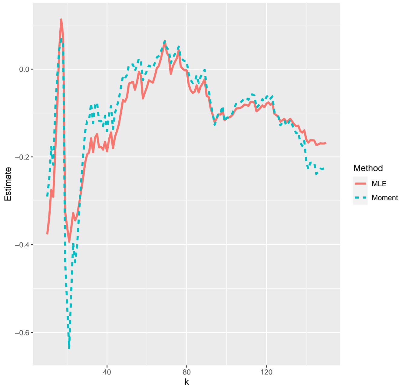
Estimates of extreme value index--18-02-2022
