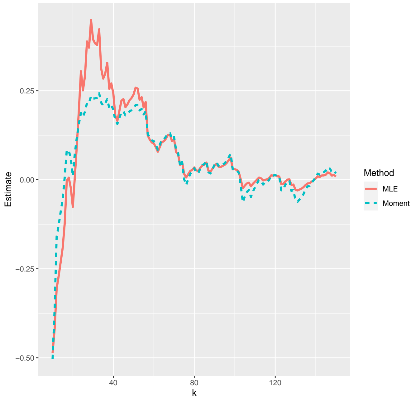
Estimates of extreme value index--17-08-2021
