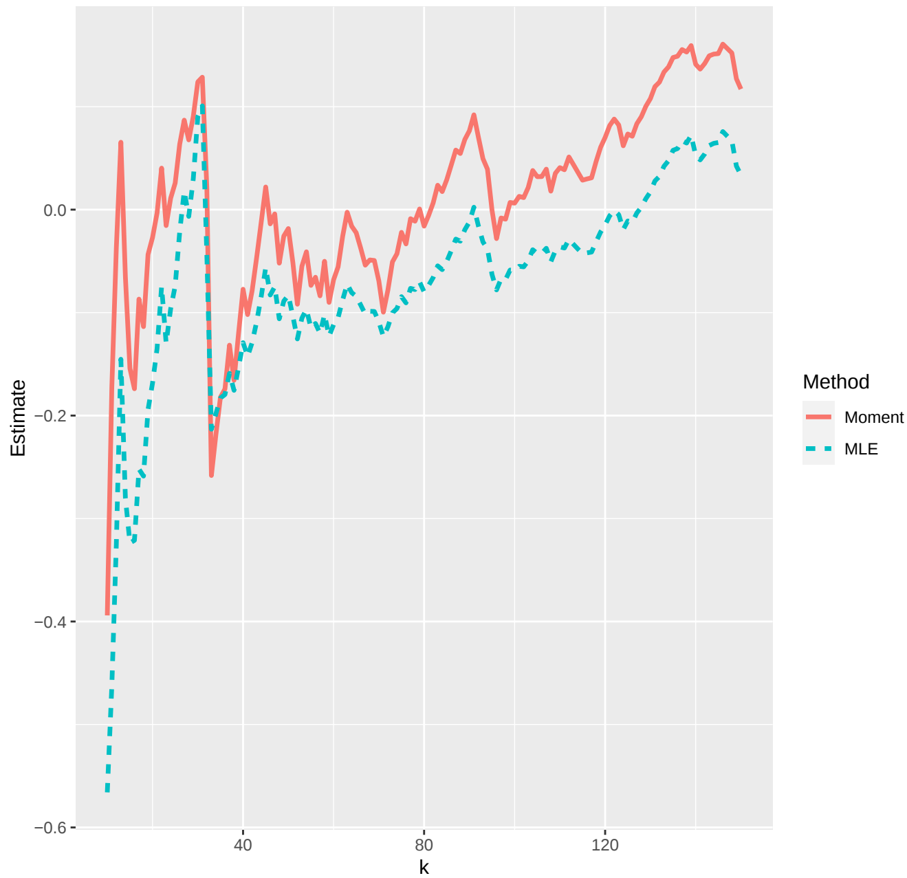
Estimates of extreme value index--17-05-2020
