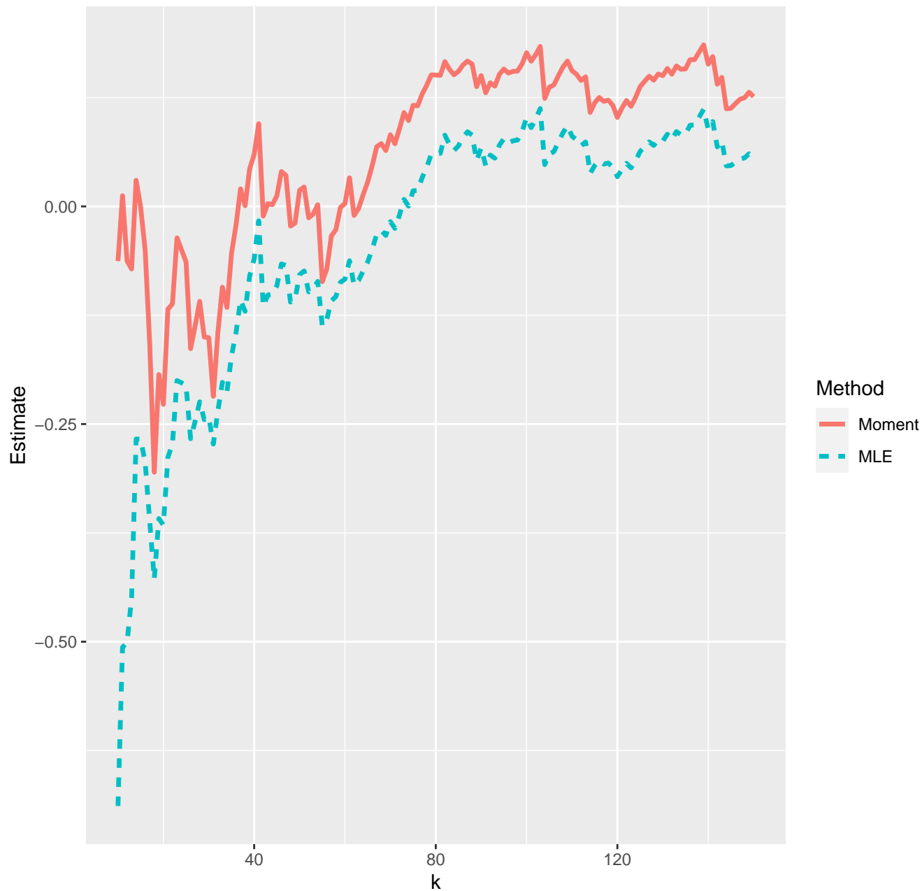
Estimates of extreme value index--17-04-2020
