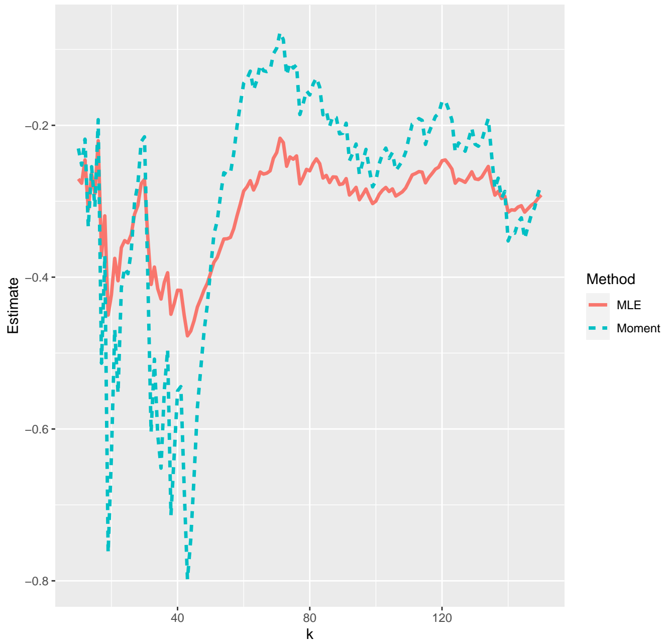
Estimates of extreme value index--16-12-2021
