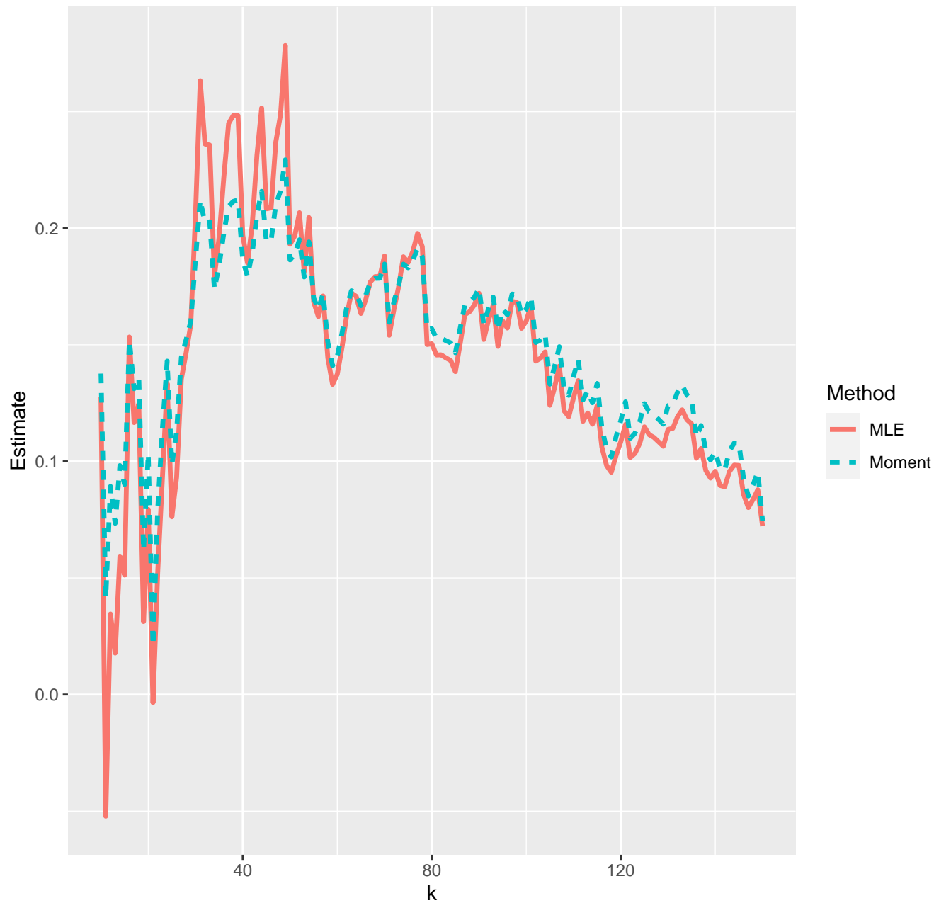
Estimates of extreme value index--16-11-2021
