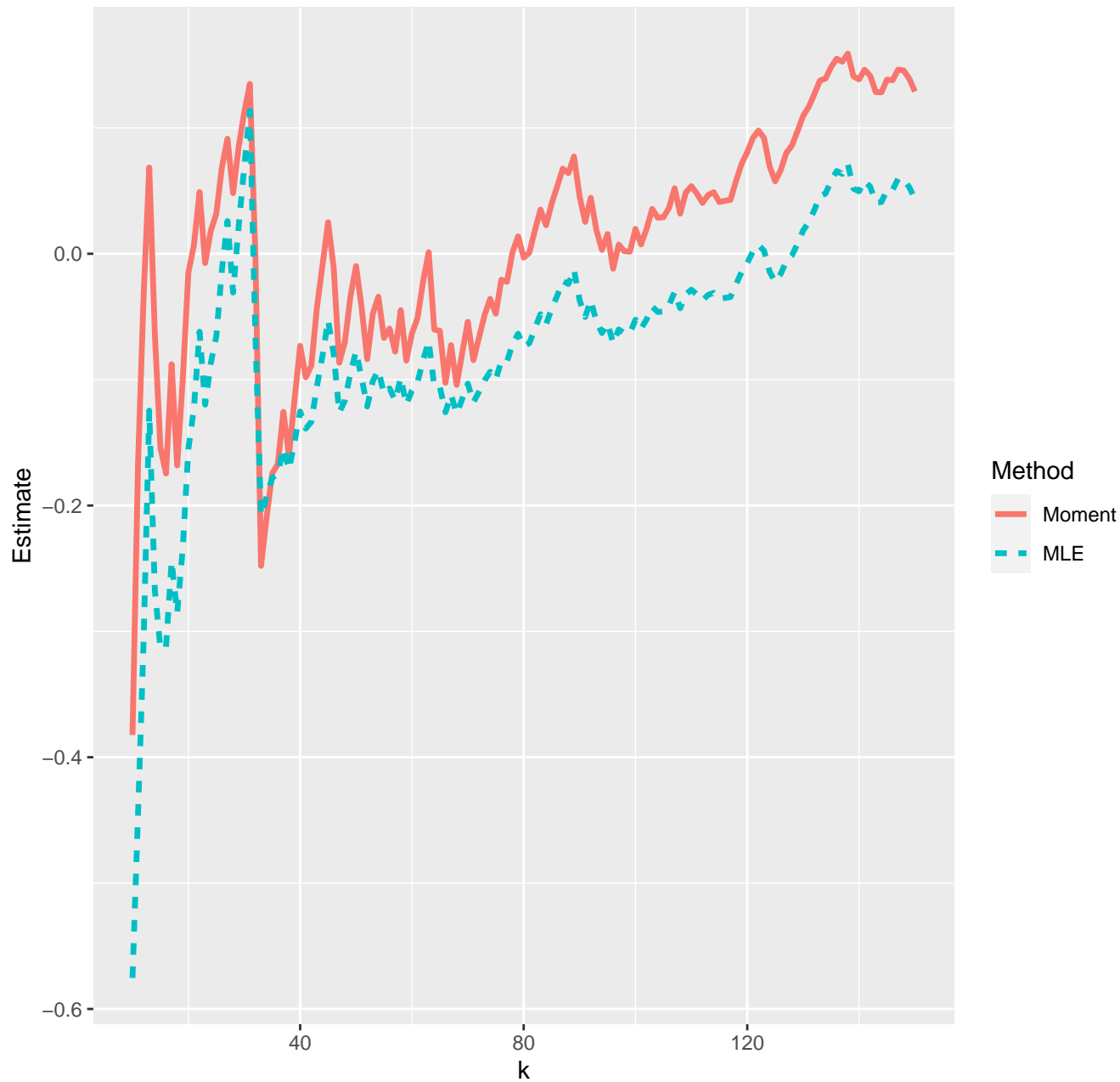
Estimates of extreme value index--16-05-2020
