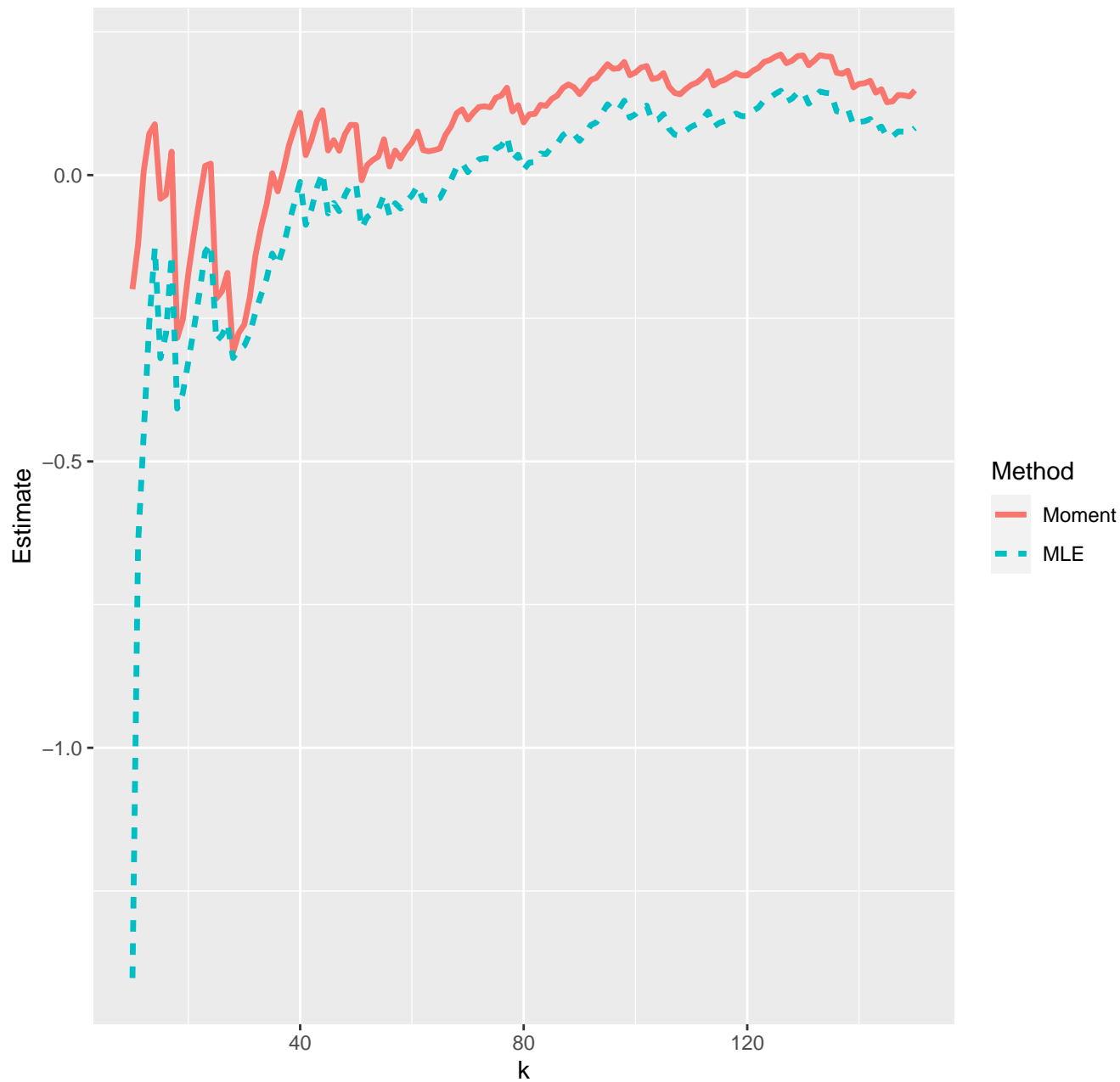
Estimates of extreme value index--16-04-2020
