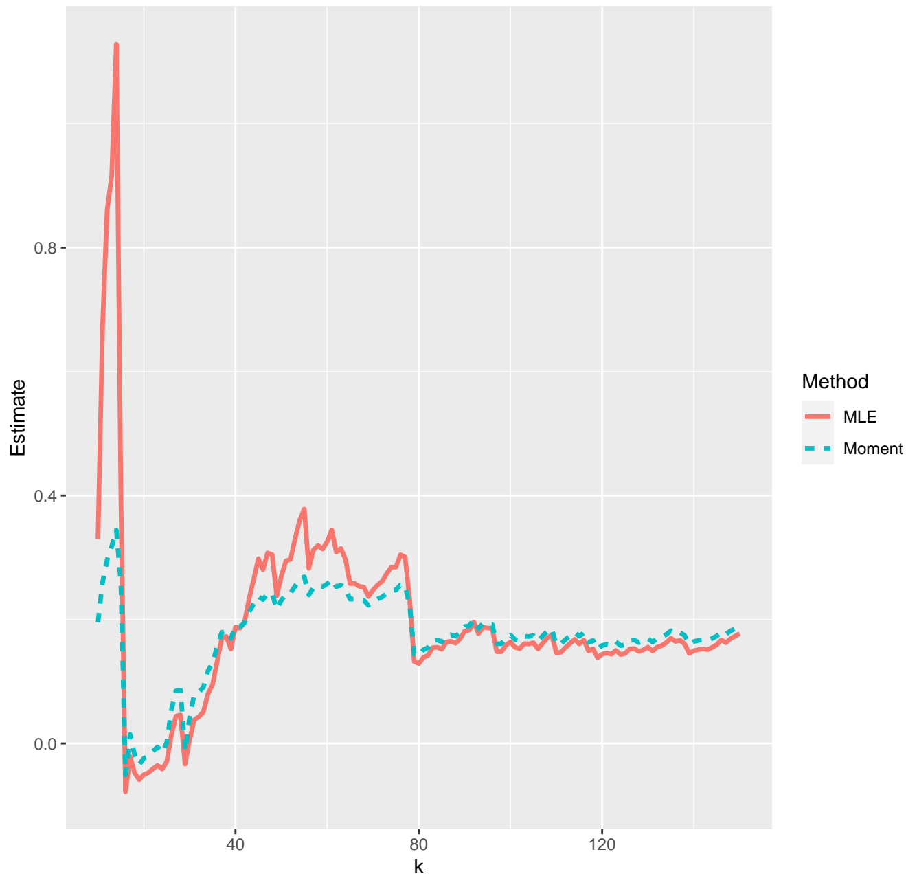
Estimates of extreme value index--15-12-2020
