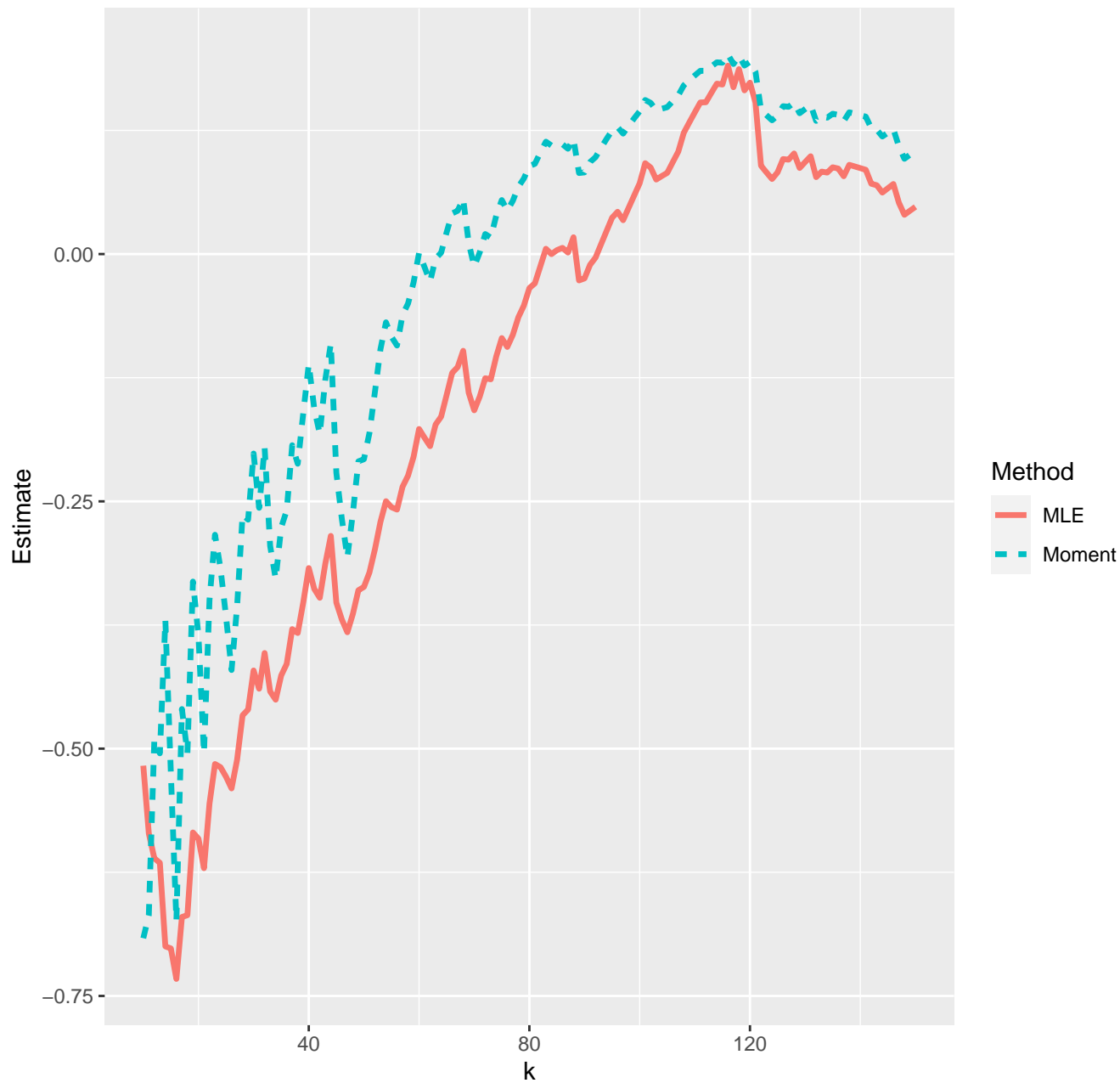
Estimates of extreme value index--15-11-2022
