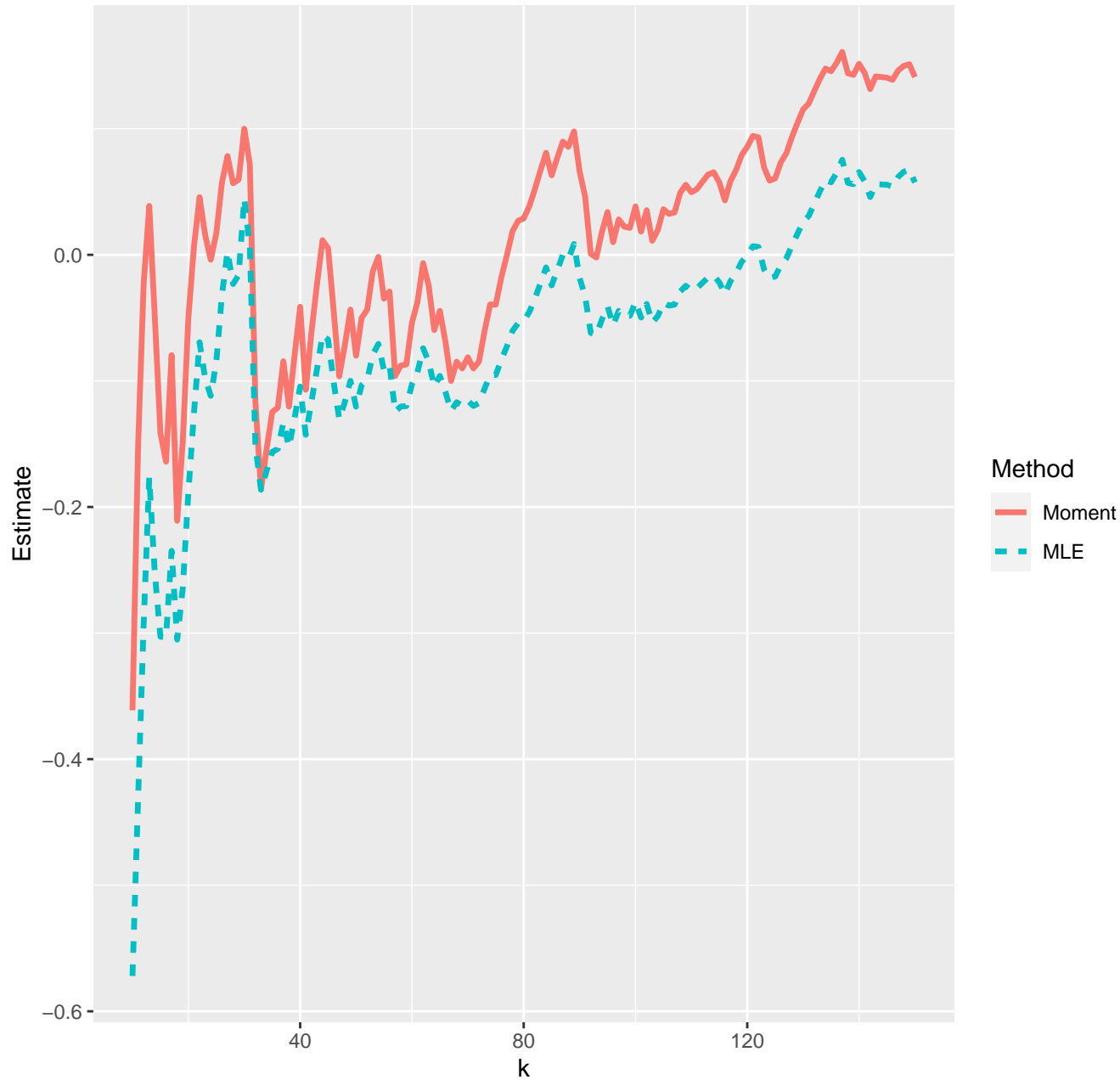
Estimates of extreme value index--15-05-2020
