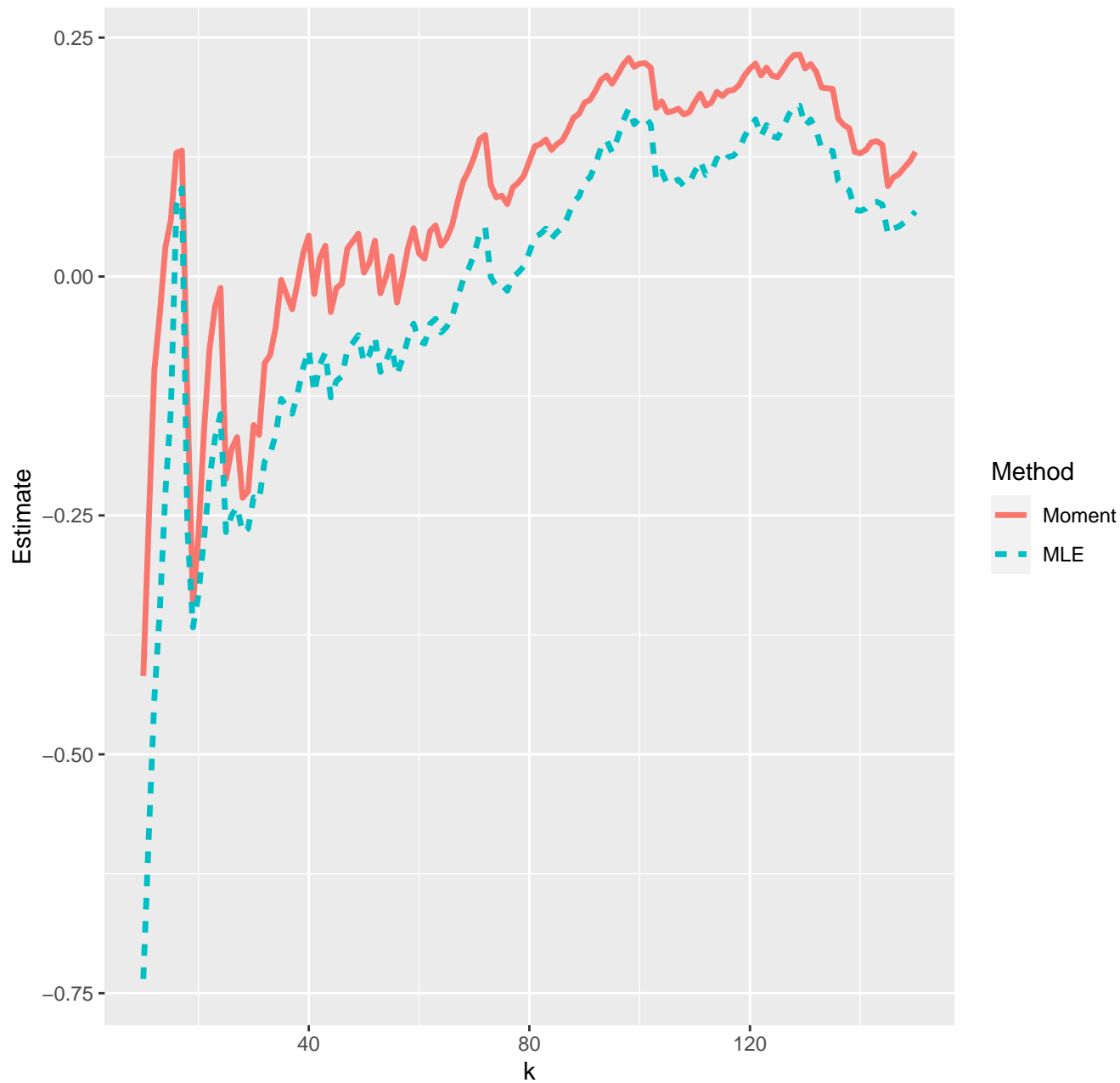
Estimates of extreme value index--15-04-2020
