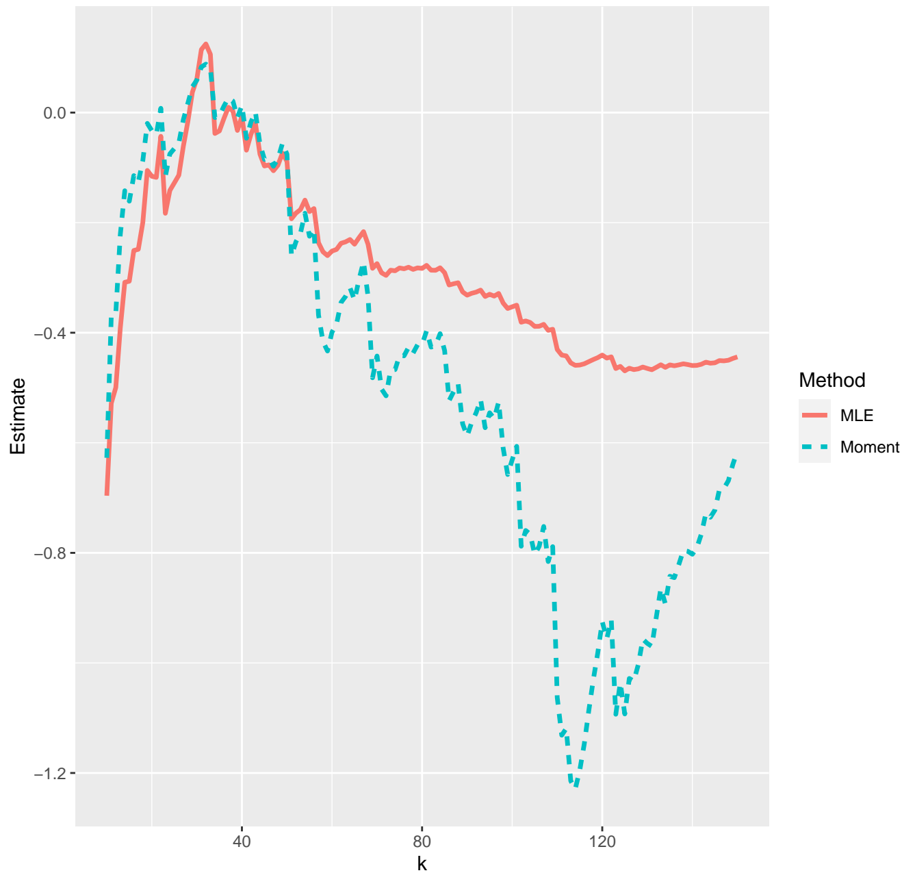
Estimates of extreme value index--15-03-2022
