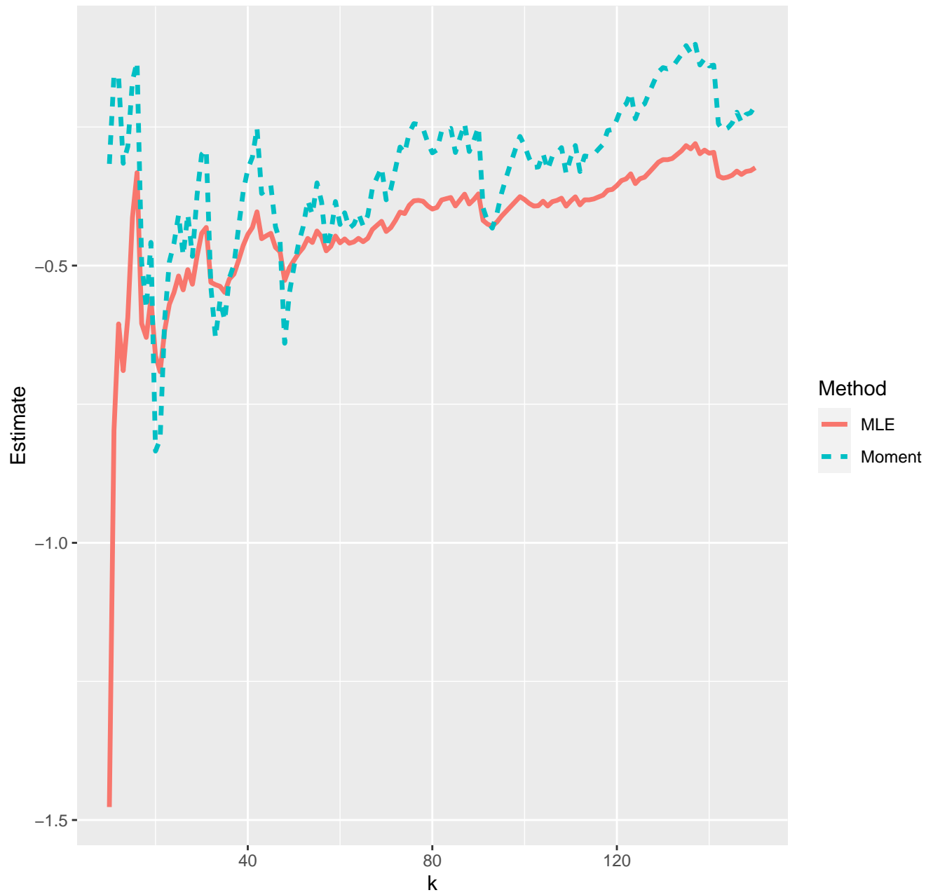
Estimates of extreme value index--14-06-2022
