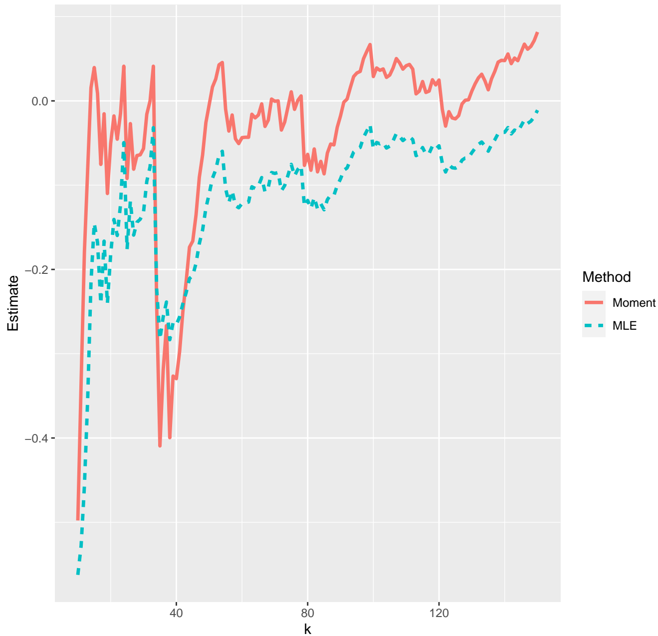
Estimates of extreme value index--14-06-2020
