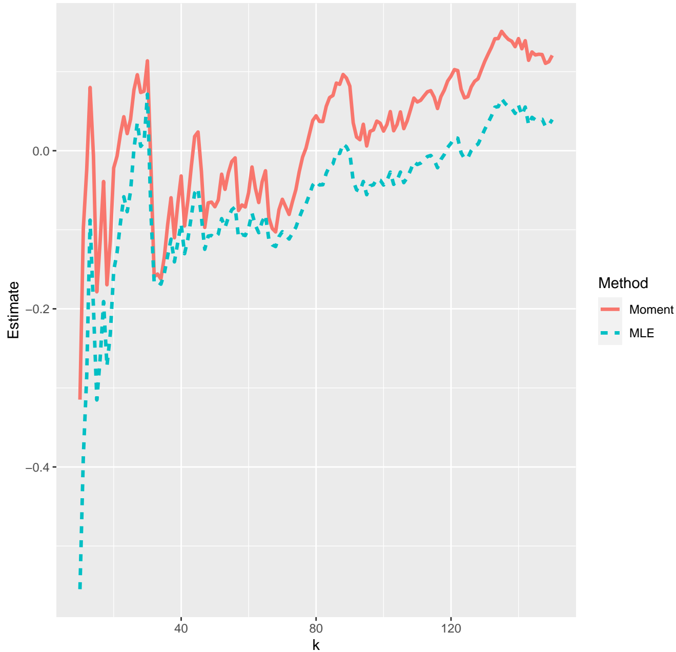
Estimates of extreme value index--14-05-2020
