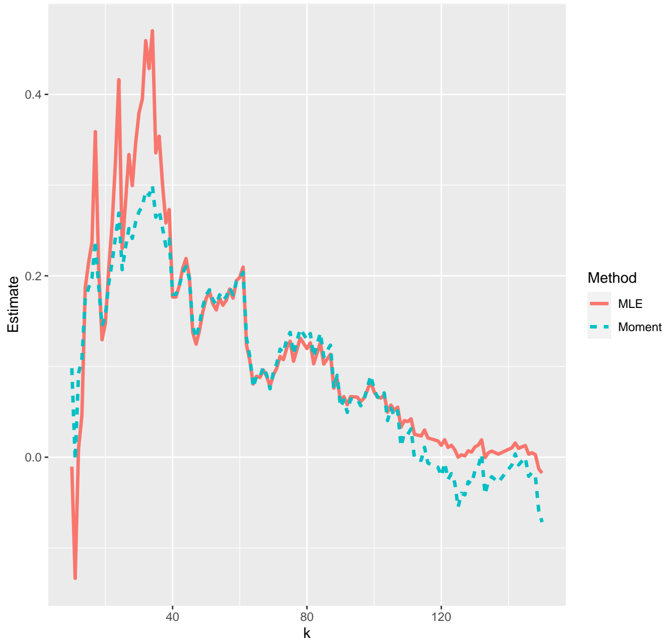
Estimates of extreme value index--13-12-2022
