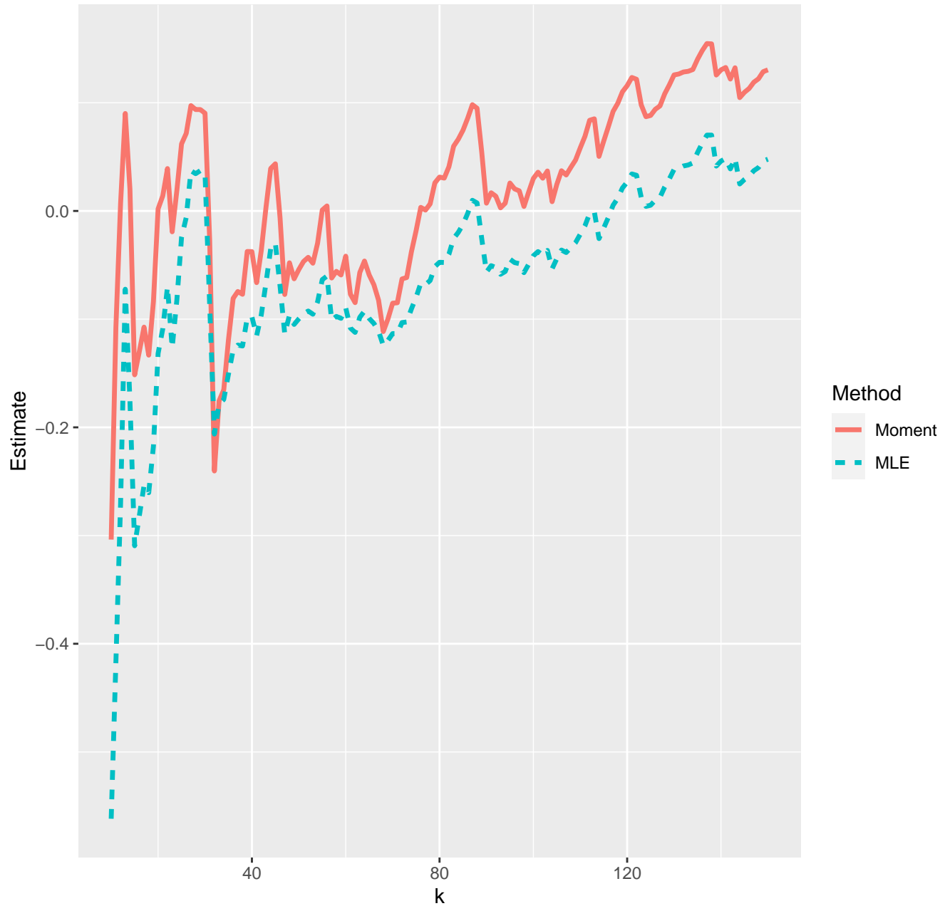
Estimates of extreme value index--13-05-2020
