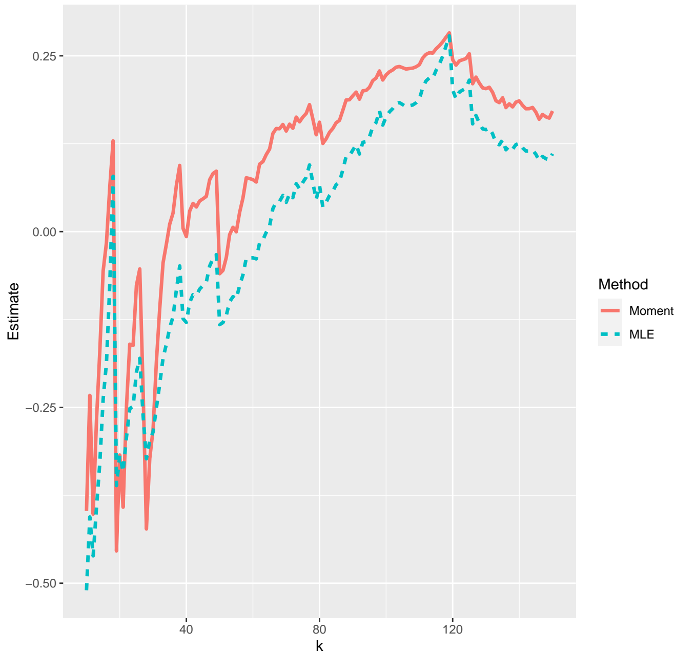
Estimates of extreme value index--13-04-2020
