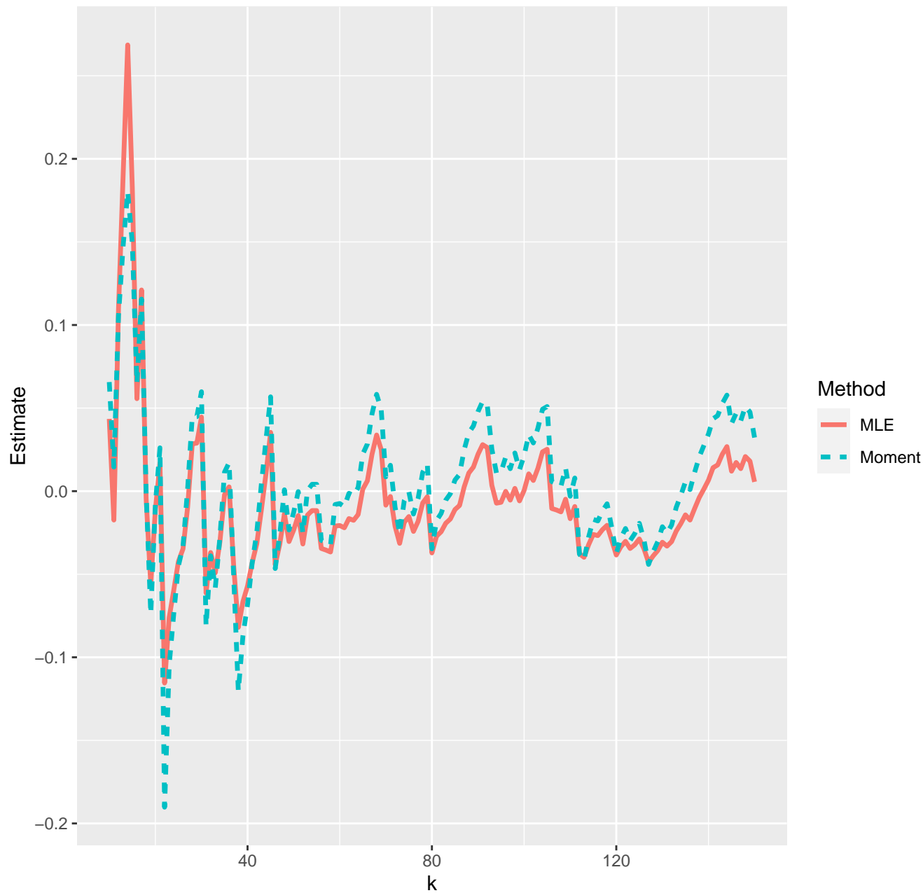
Estimates of extreme value index--13-01-2022
