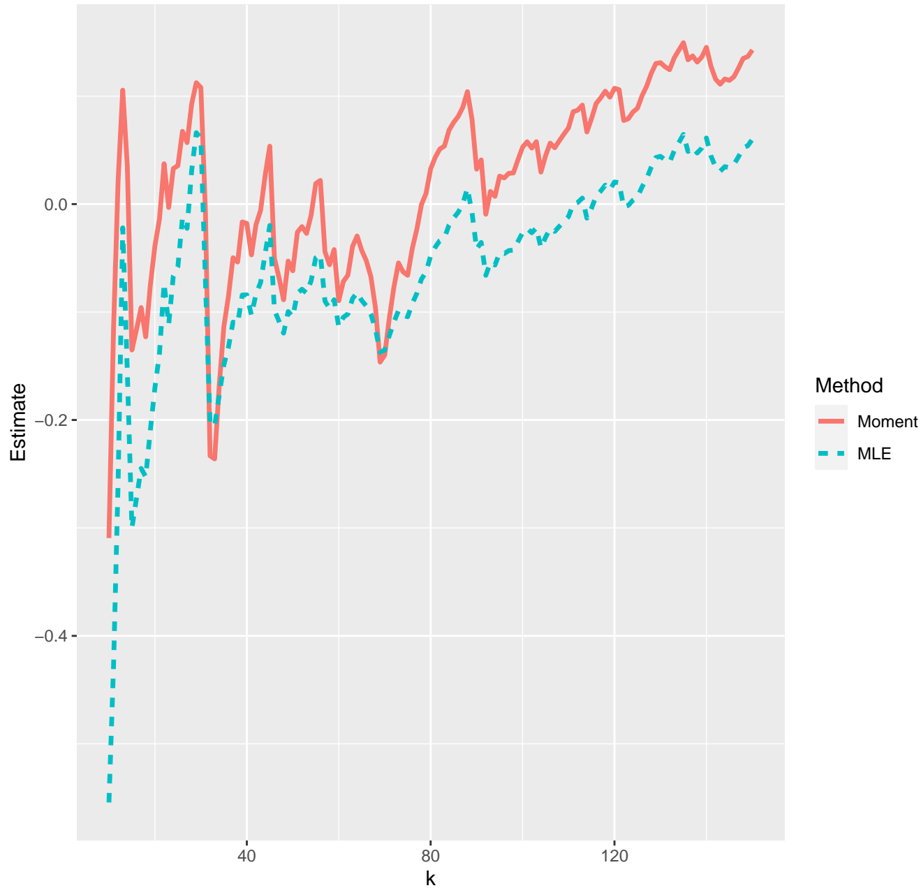
Estimates of extreme value index--12-05-2020
