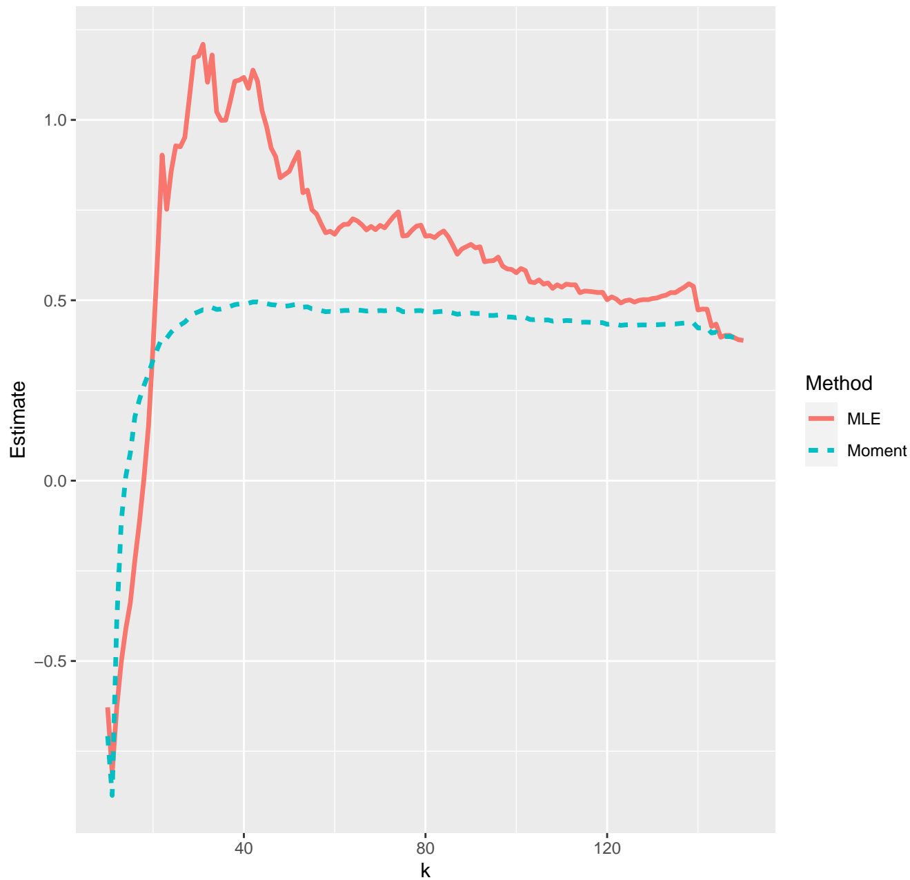
Estimates of extreme value index--12-04-2022
