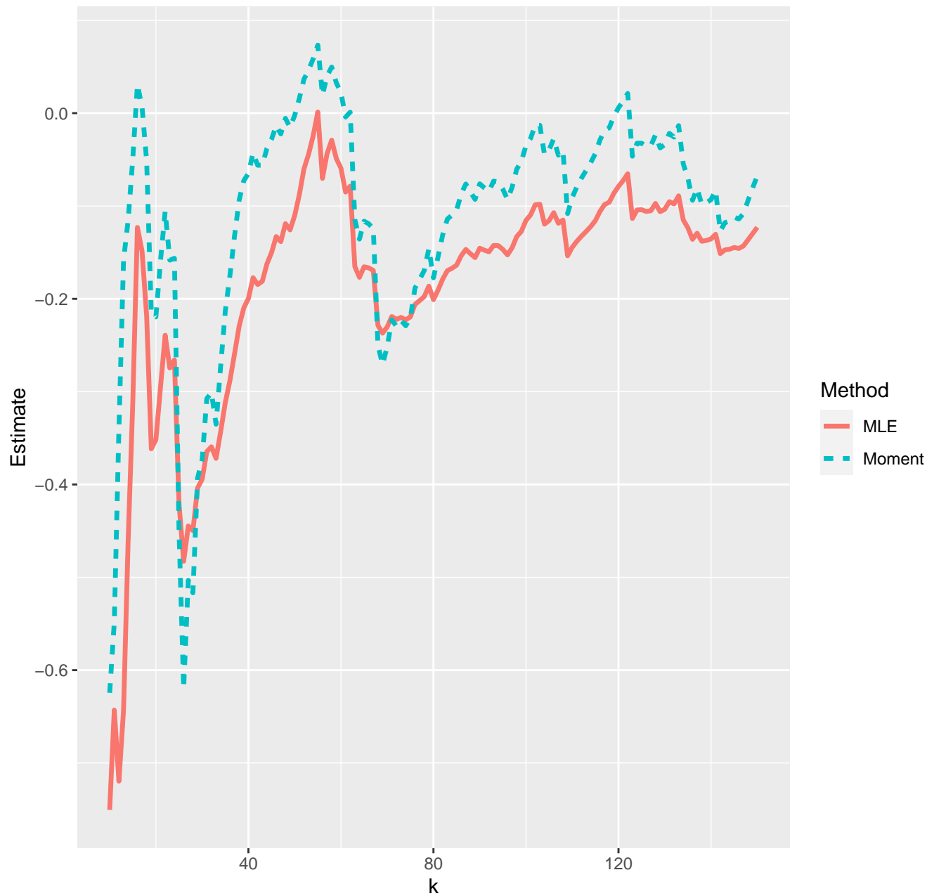
Estimates of extreme value index--12-01-2021
