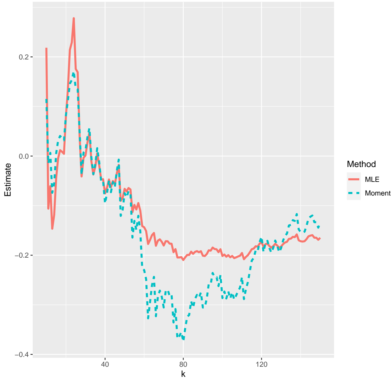
Estimates of extreme value index--11-05-2021
