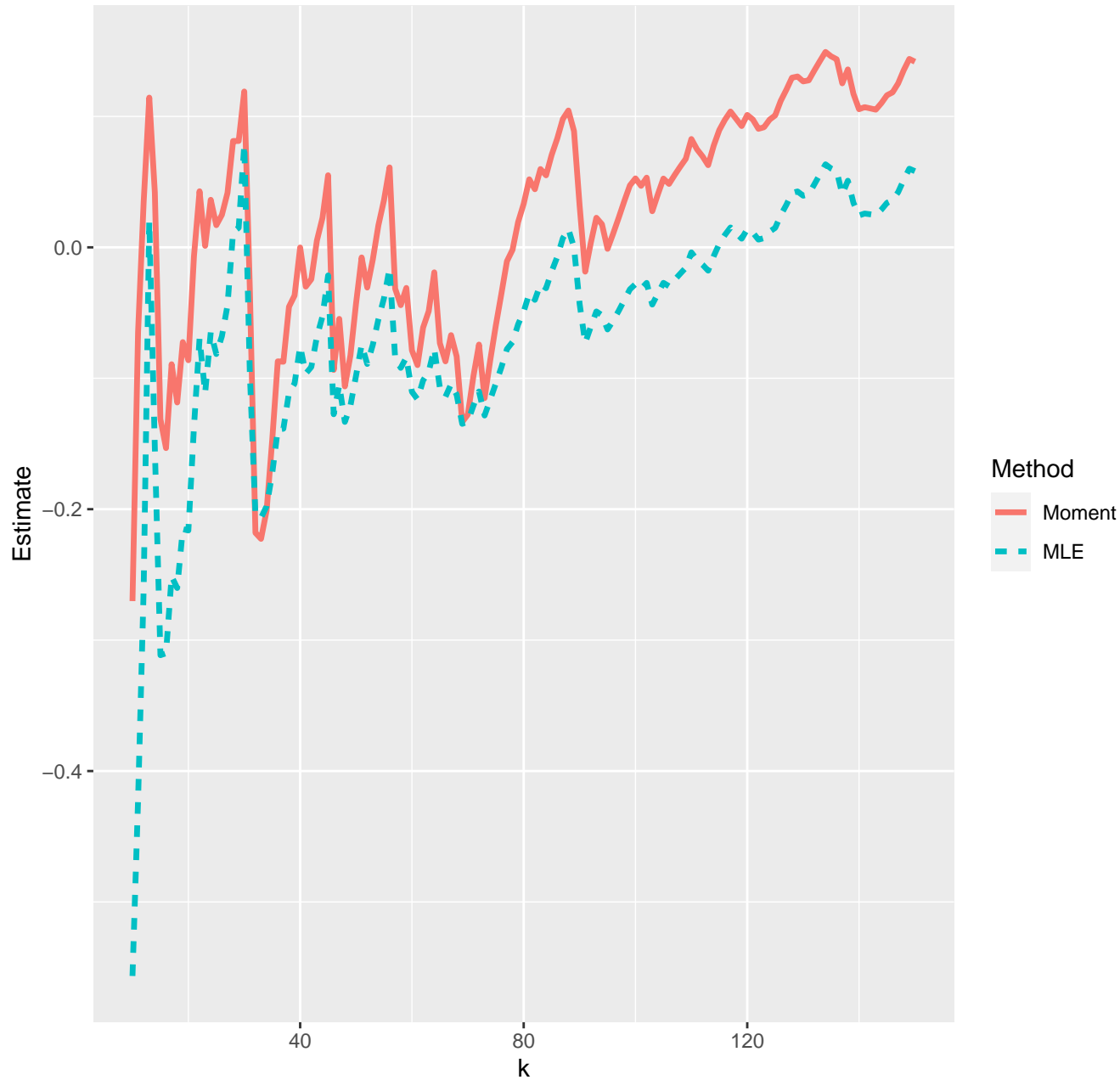
Estimates of extreme value index--11-05-2020
