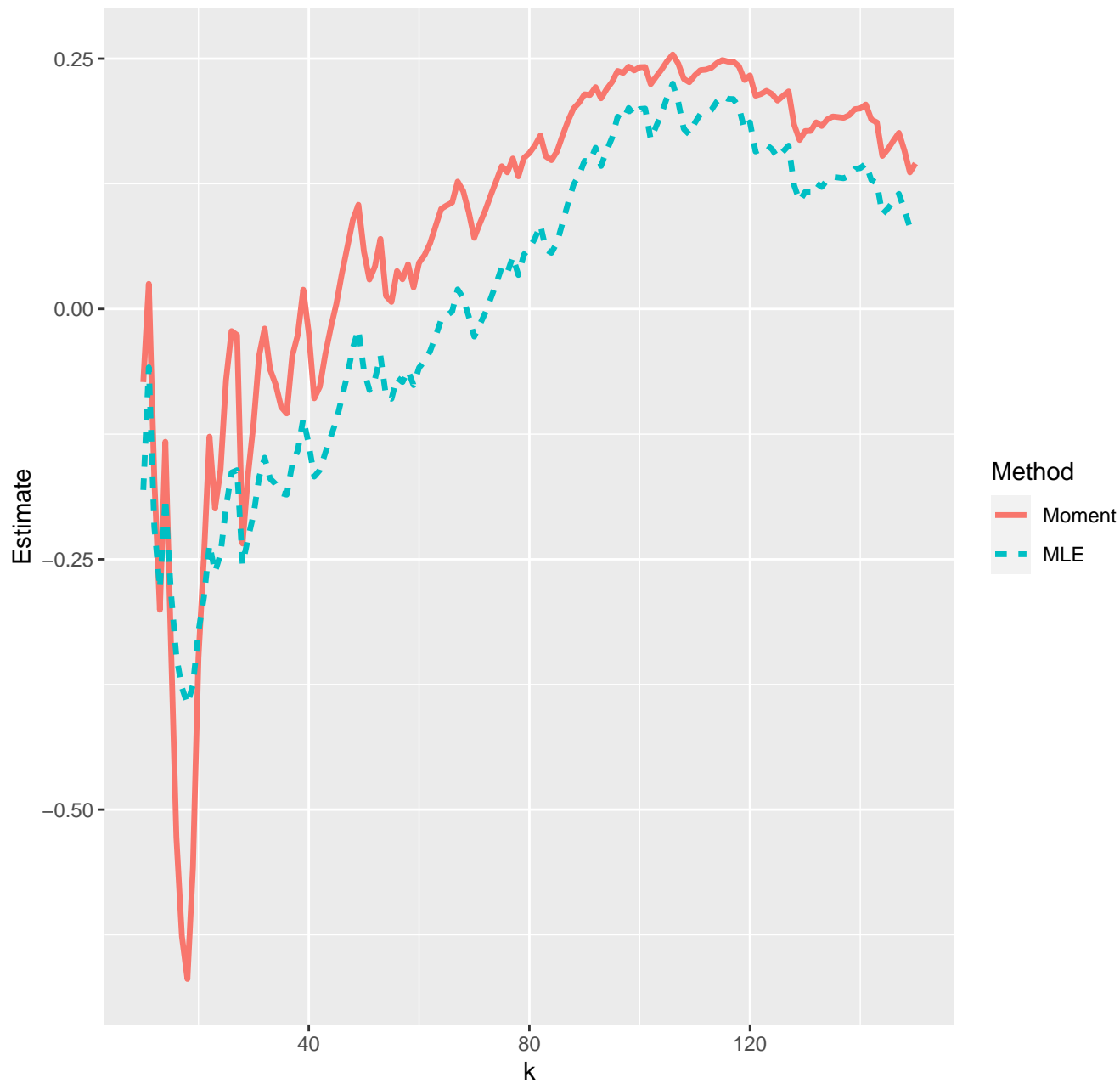
Estimates of extreme value index--11-04-2020
