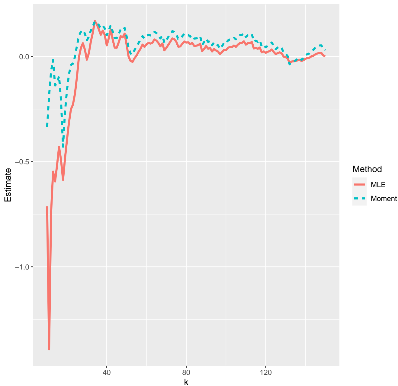
Estimates of extreme value index--10-11-2021
