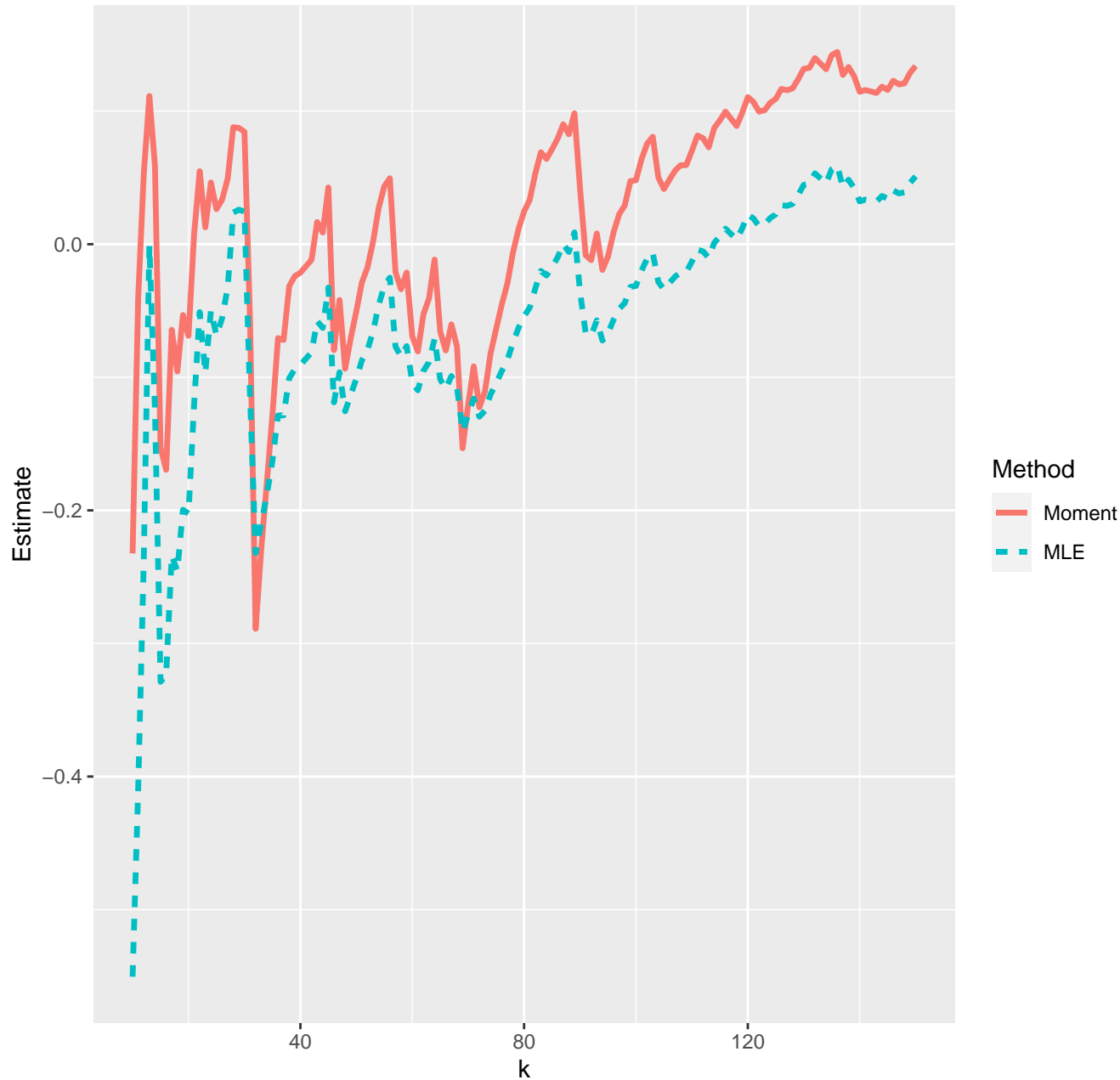
Estimates of extreme value index--10-05-2020
