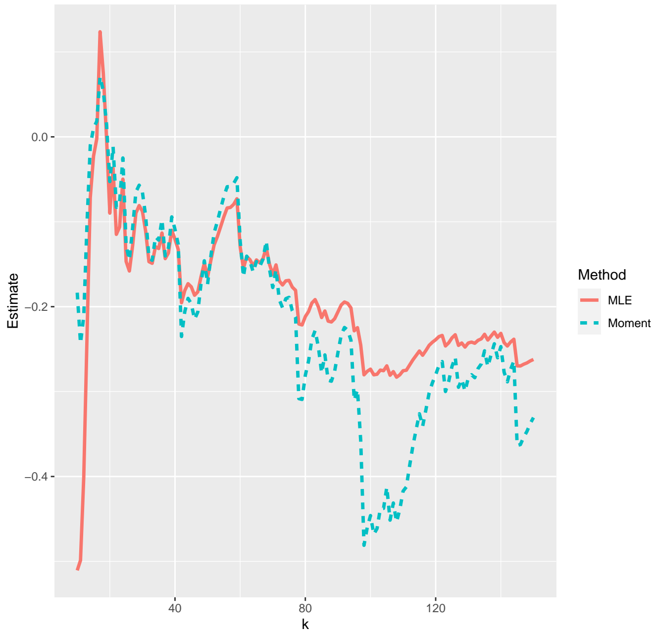
Estimates of extreme value index--10-02-2022
