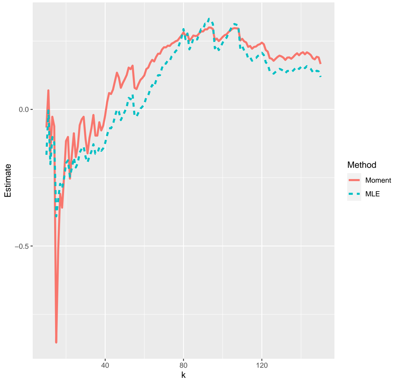
Estimates of extreme value index--09-04-2020
