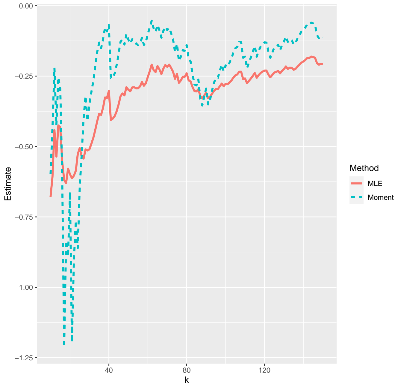
Estimates of extreme value index--09-02-2021
