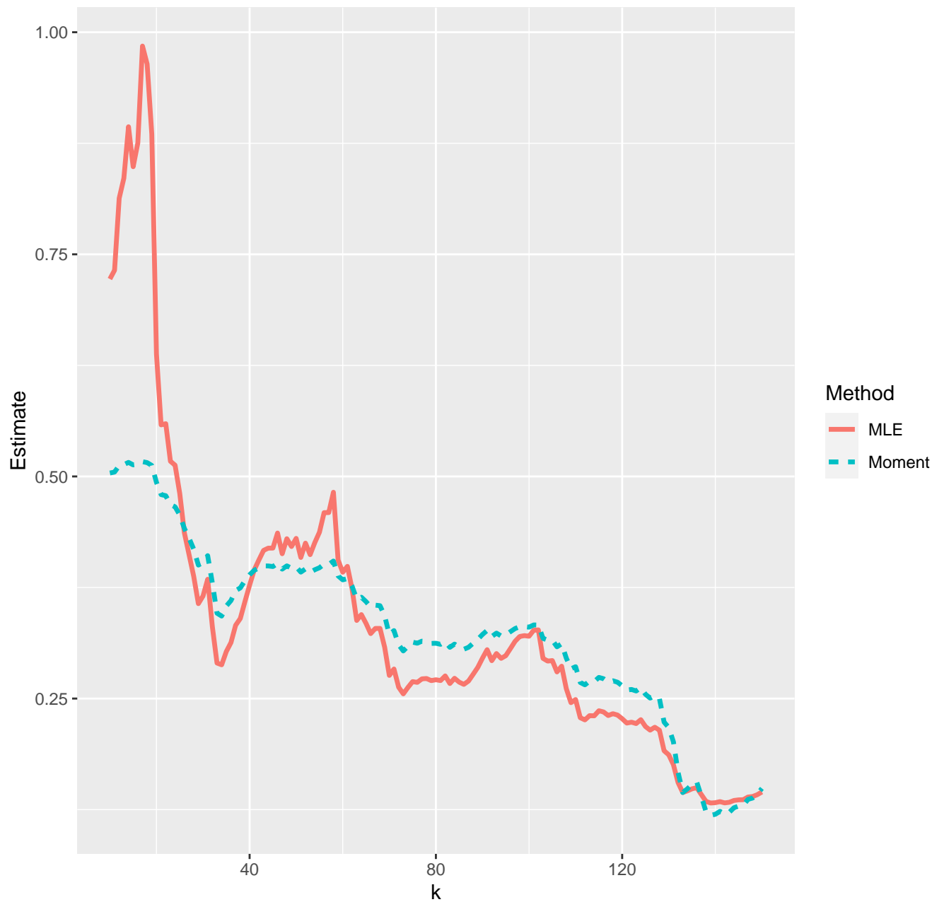
Estimates of extreme value index--08-12-2020
