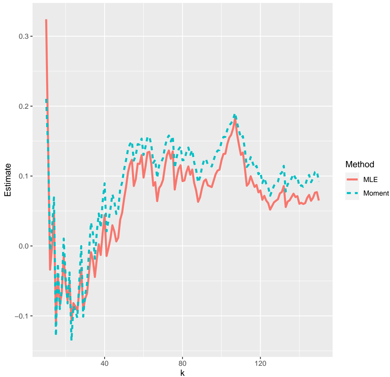
Estimates of extreme value index--08-11-2022
