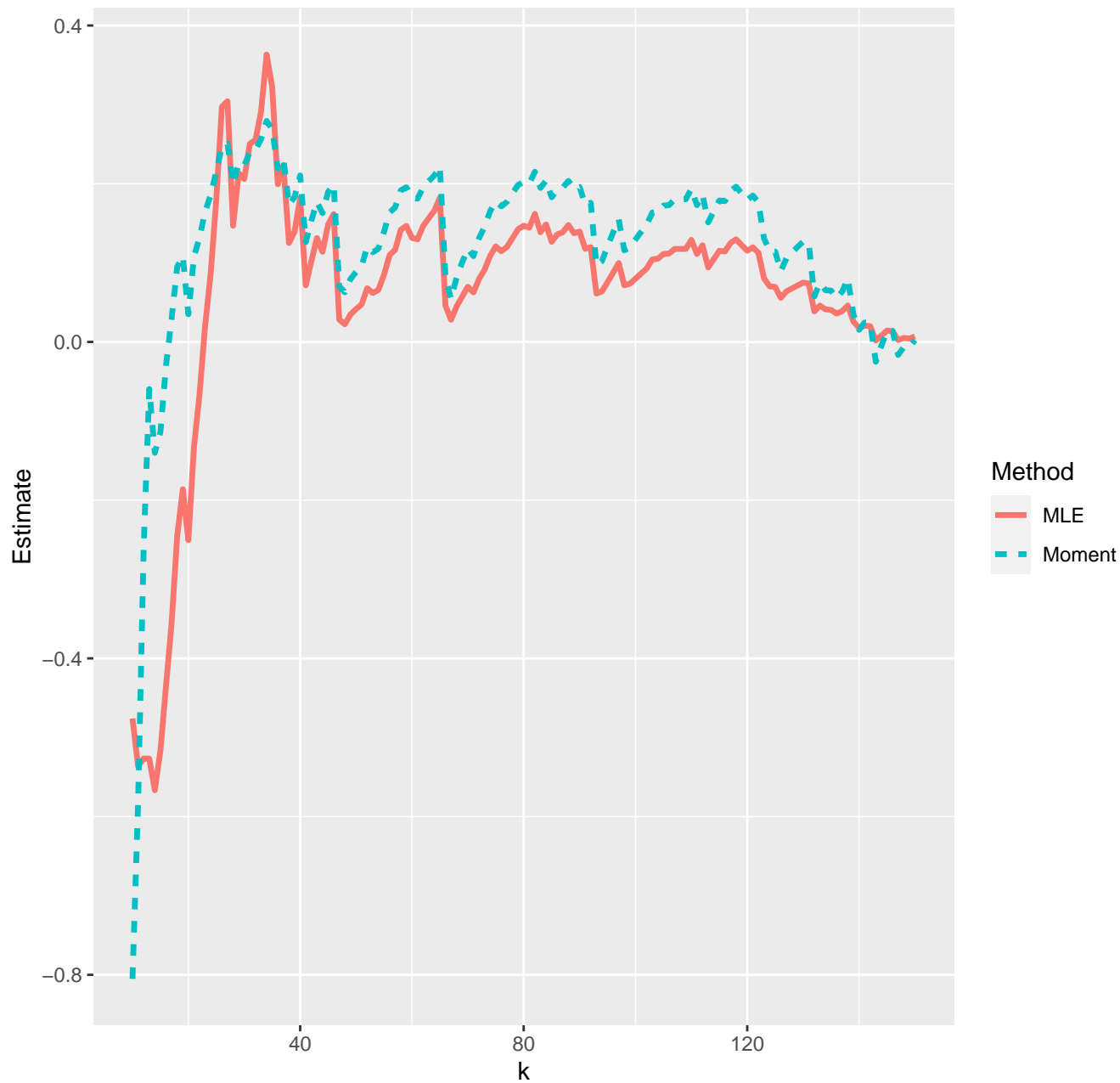
Estimates of extreme value index--08-09-2020
