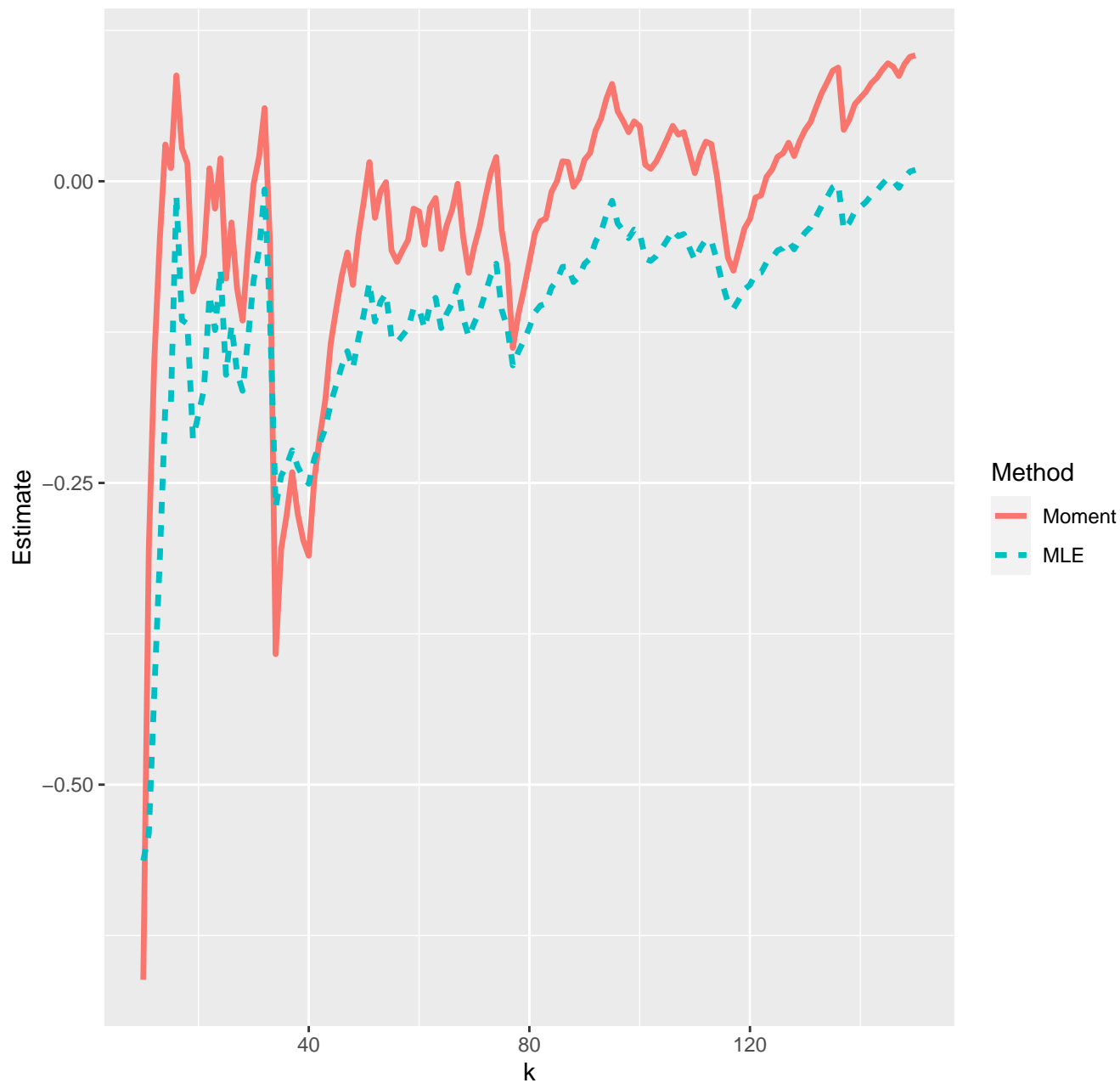
Estimates of extreme value index--08-06-2020
