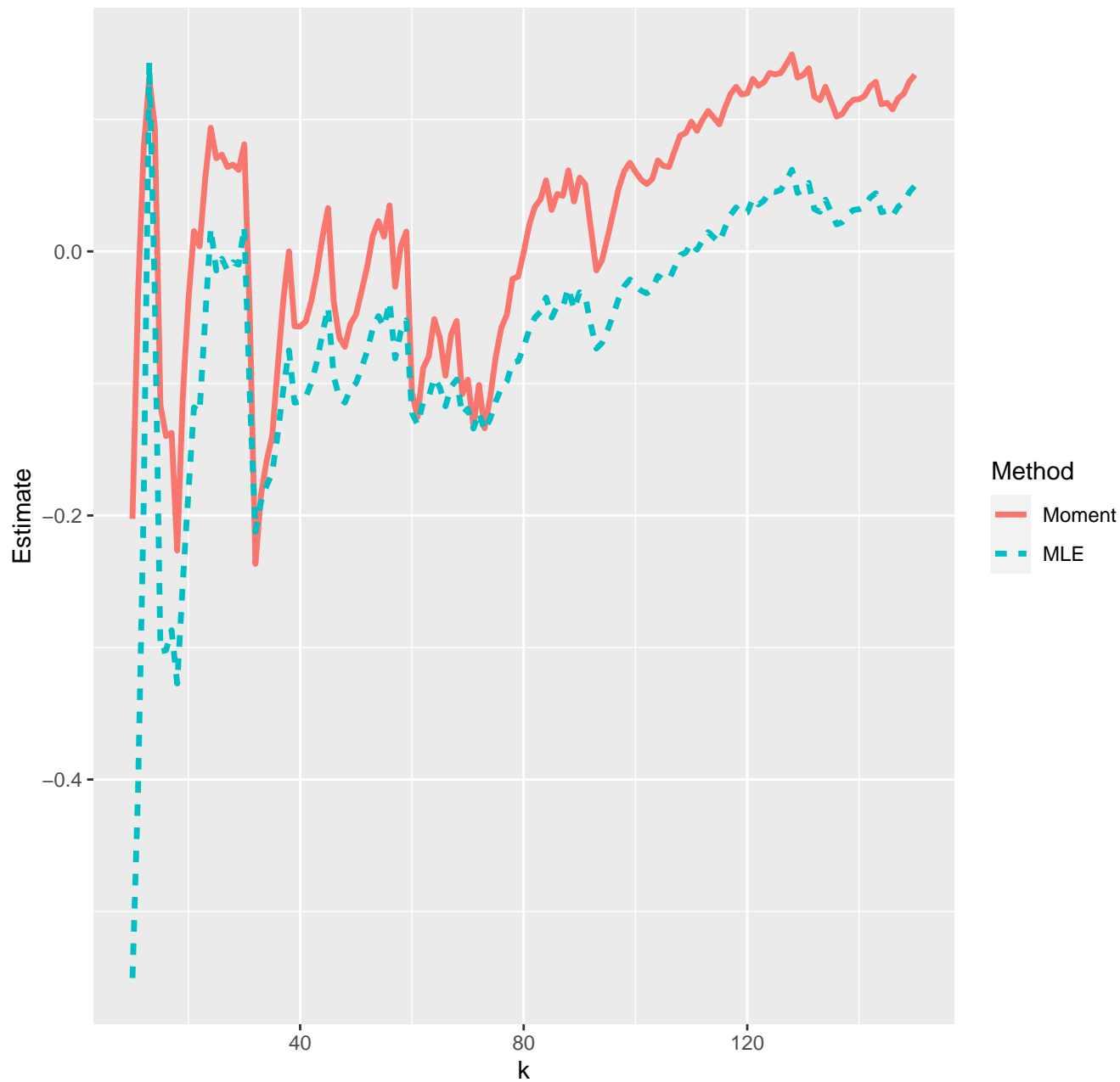
Estimates of extreme value index--08-05-2020
