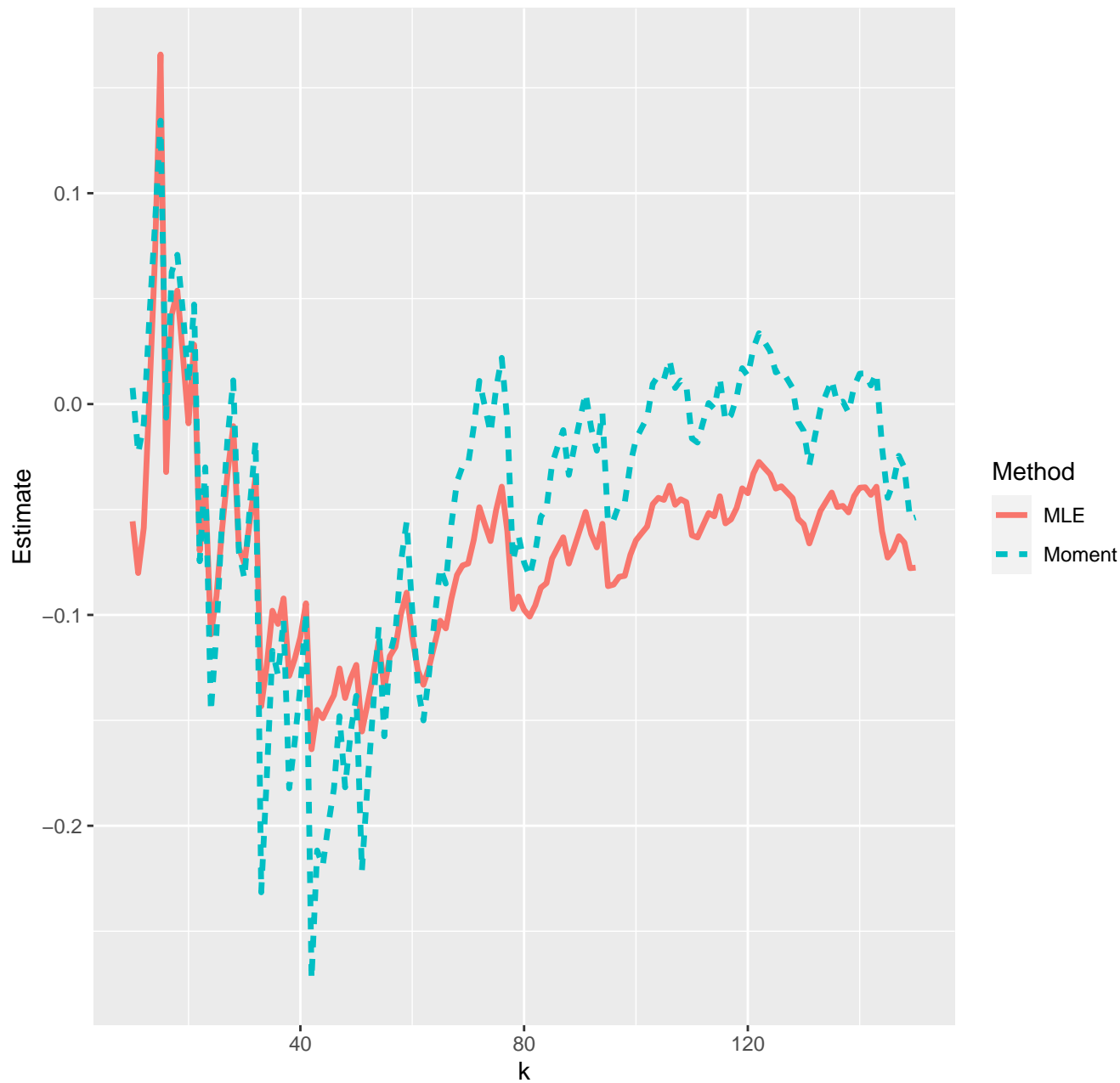
Estimates of extreme value index--07-06-2022
