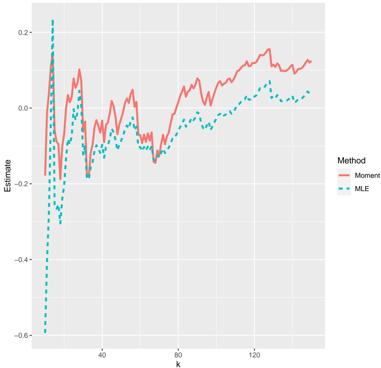
Estimates of extreme value index--07-05-2020
