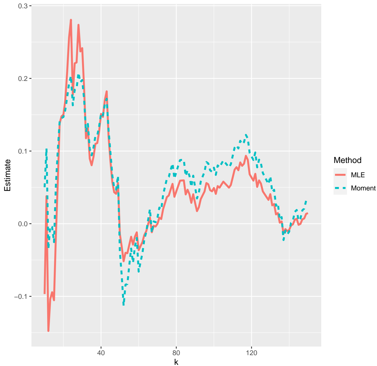
Estimates of extreme value index--06-12-2022
