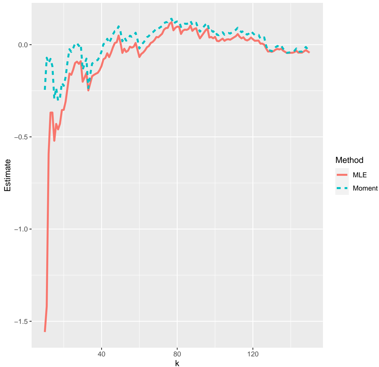
Estimates of extreme value index--06-09-2022
