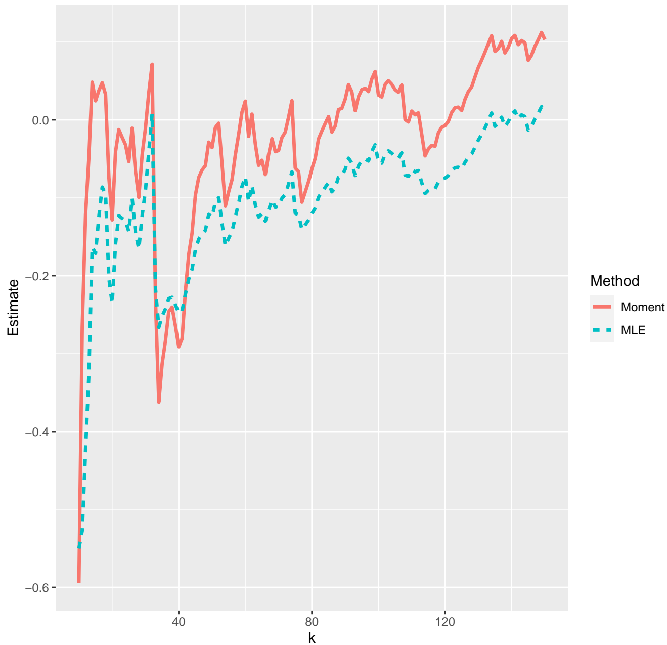
Estimates of extreme value index--06-06-2020
