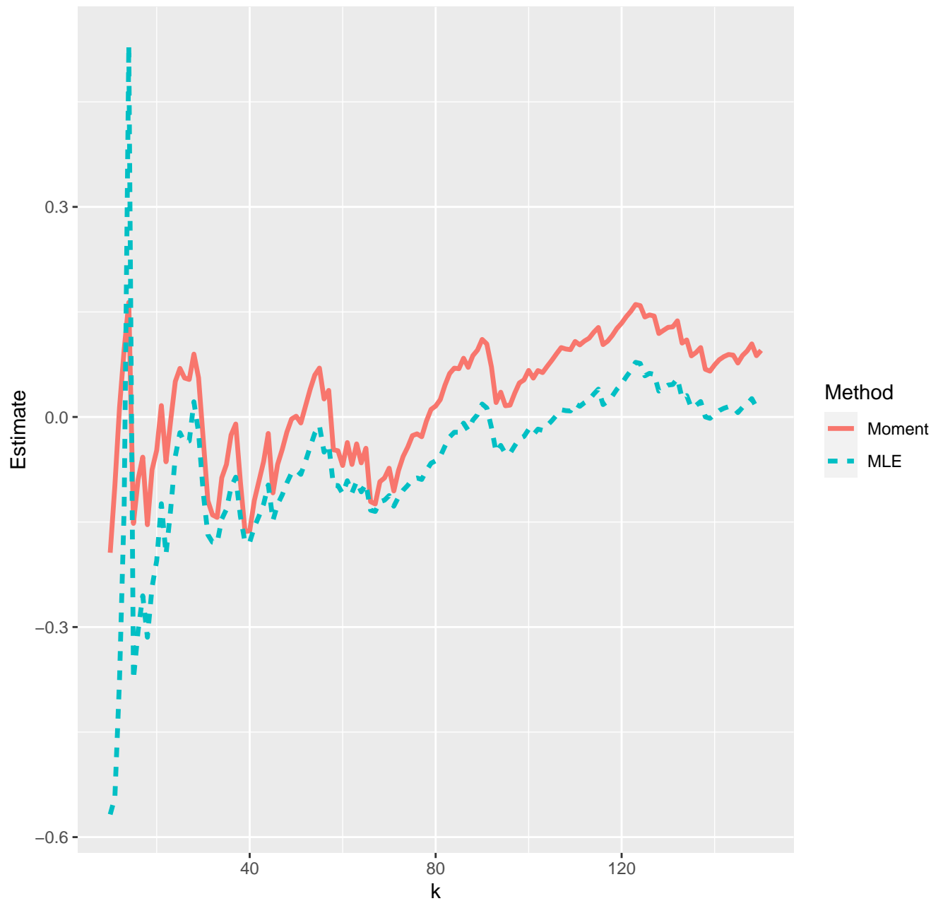
Estimates of extreme value index--06-05-2020
