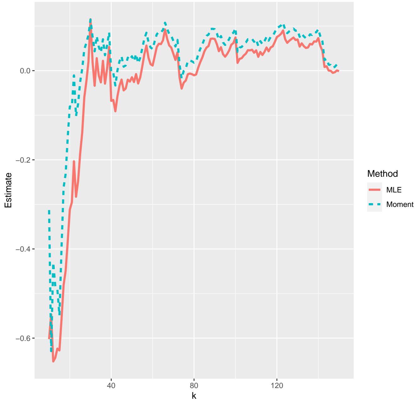
Estimates of extreme value index--06-04-2021
