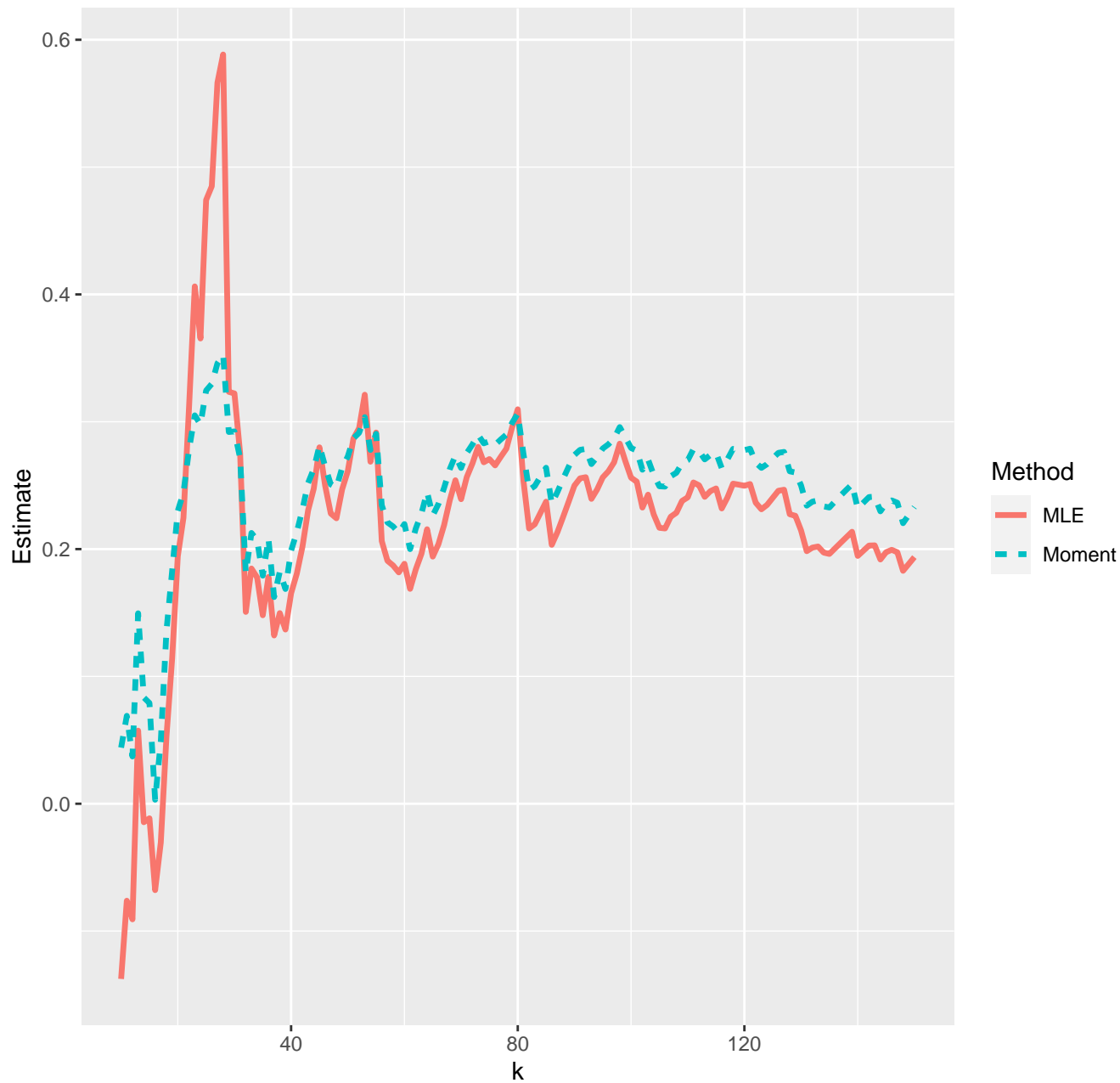
Estimates of extreme value index--05-10-2021
