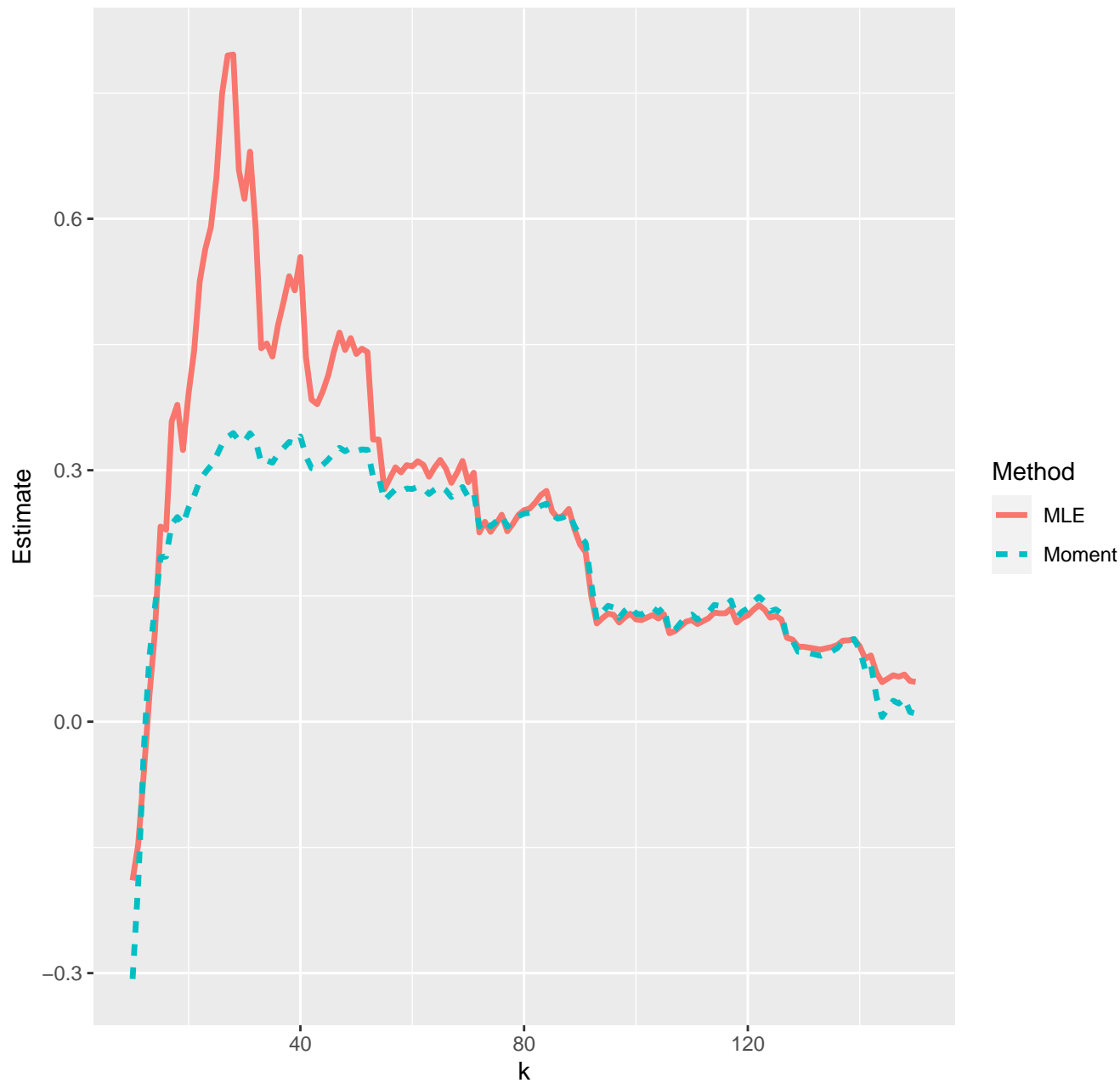
Estimates of extreme value index--05-07-2022
