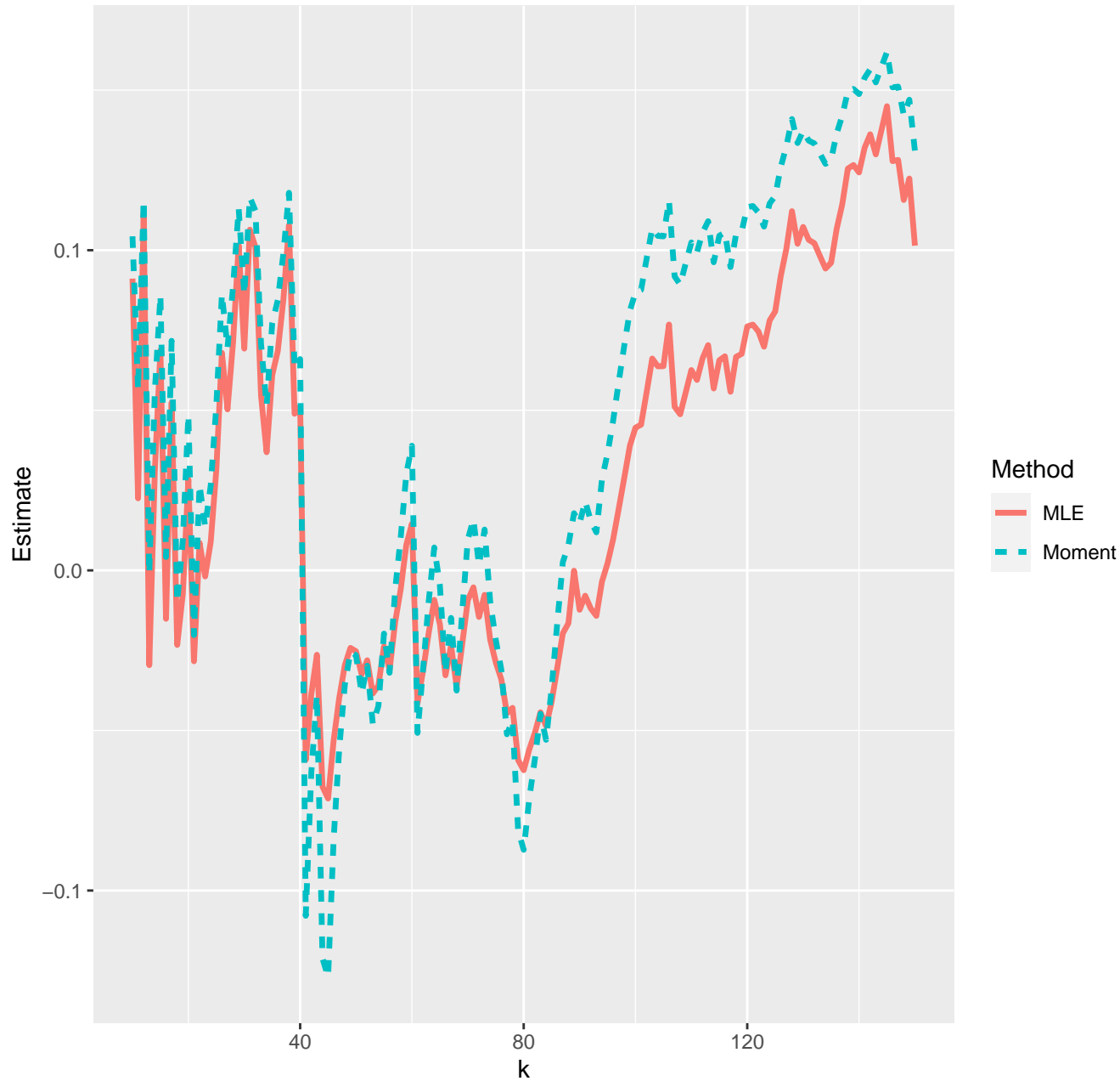
Estimates of extreme value index--04-10-2022
