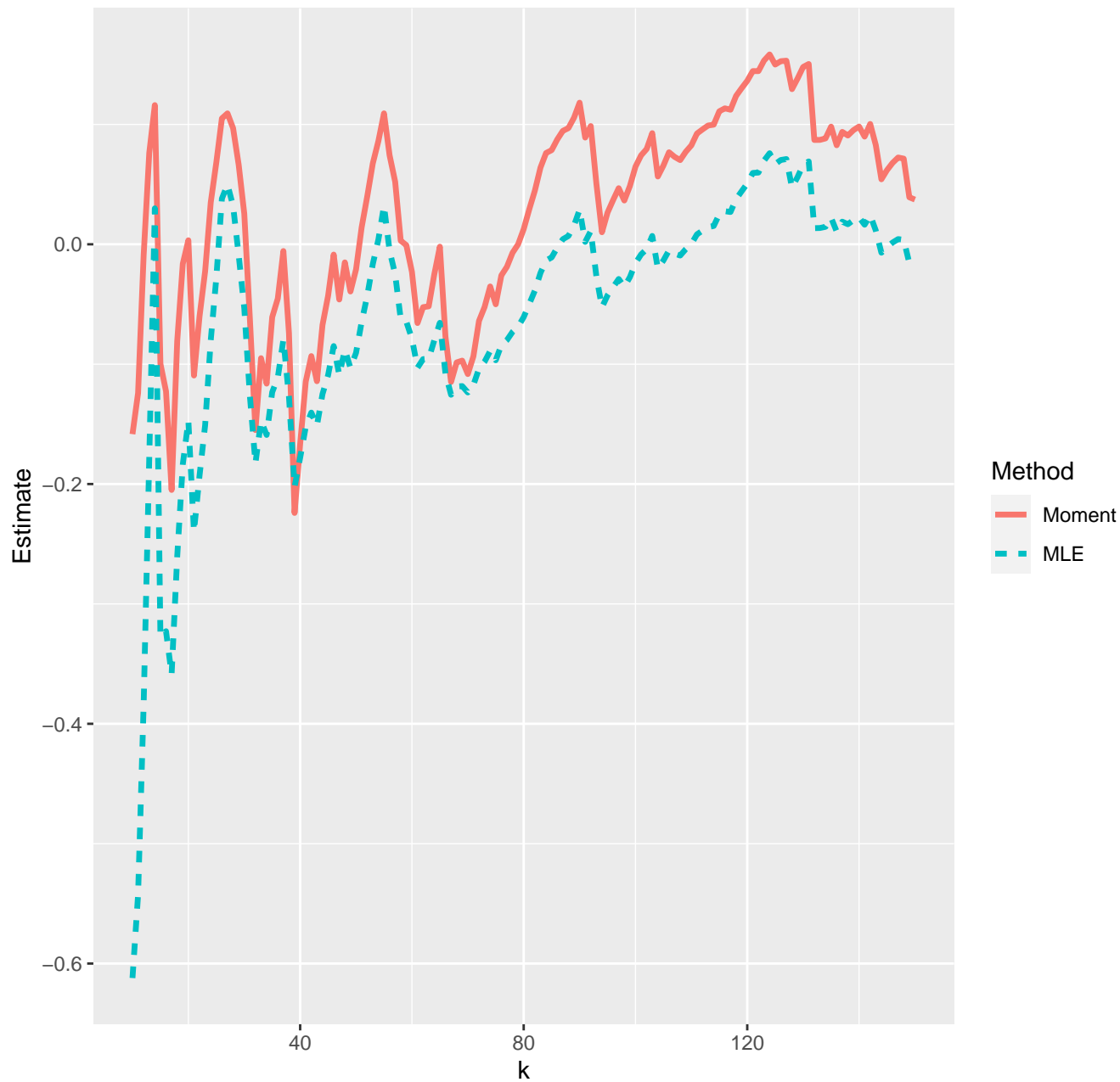
Estimates of extreme value index--04-05-2020
